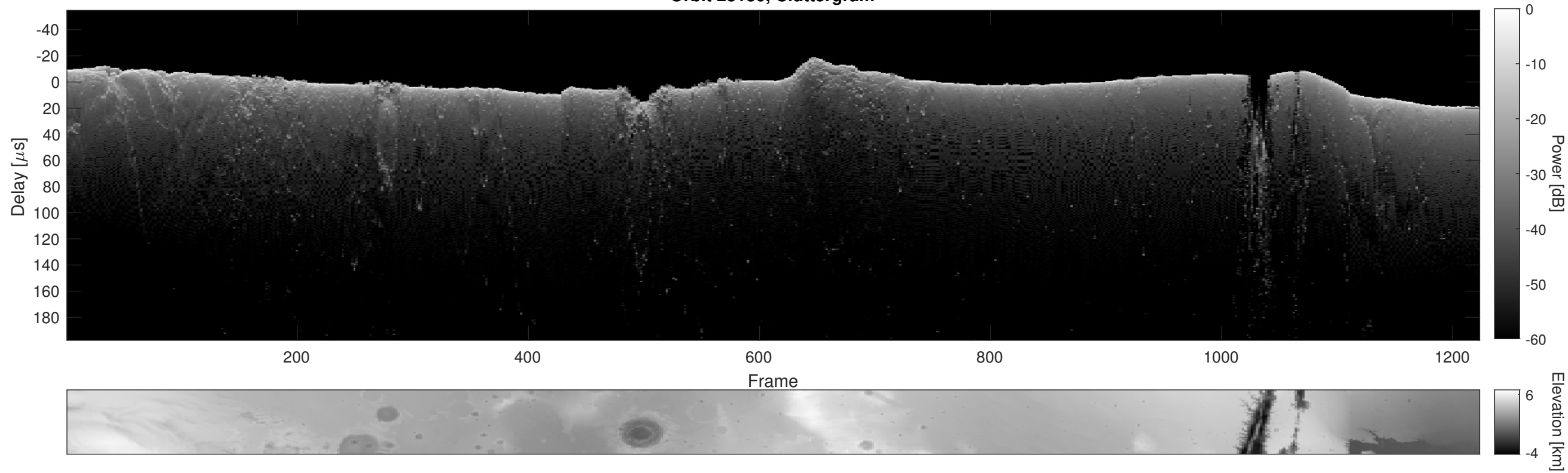
Orbit 23130, Cluttergram
