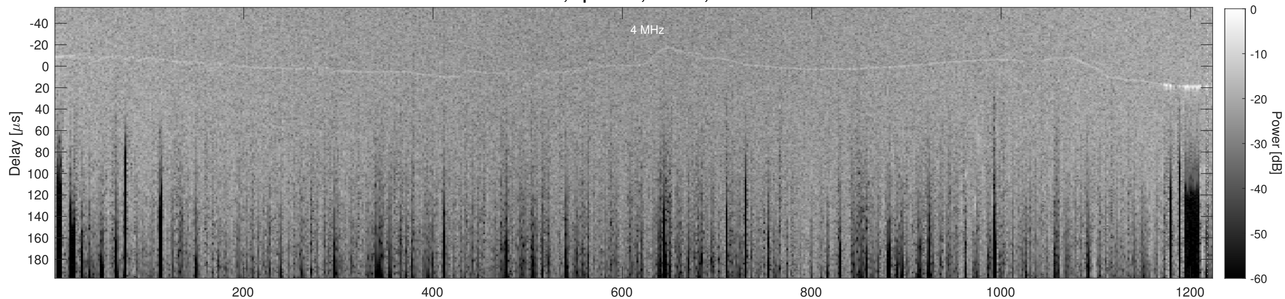
Orbit 23130, Cluttergram
