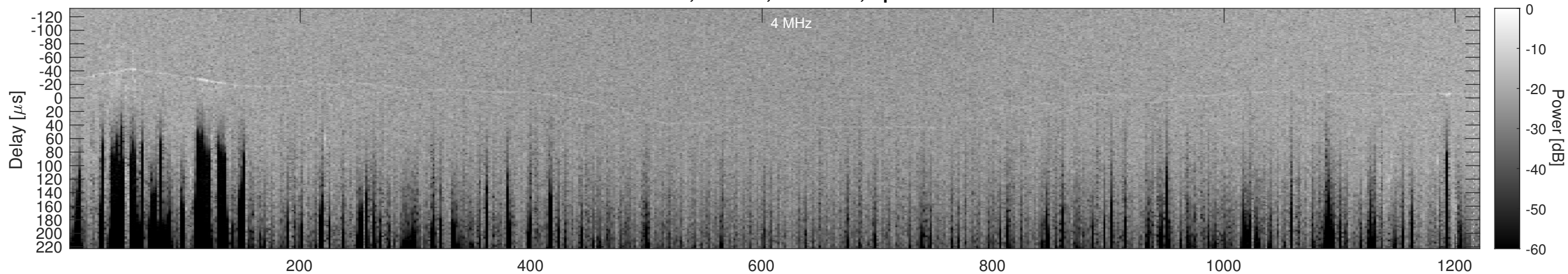
Orbit 23132, Cluttergram
