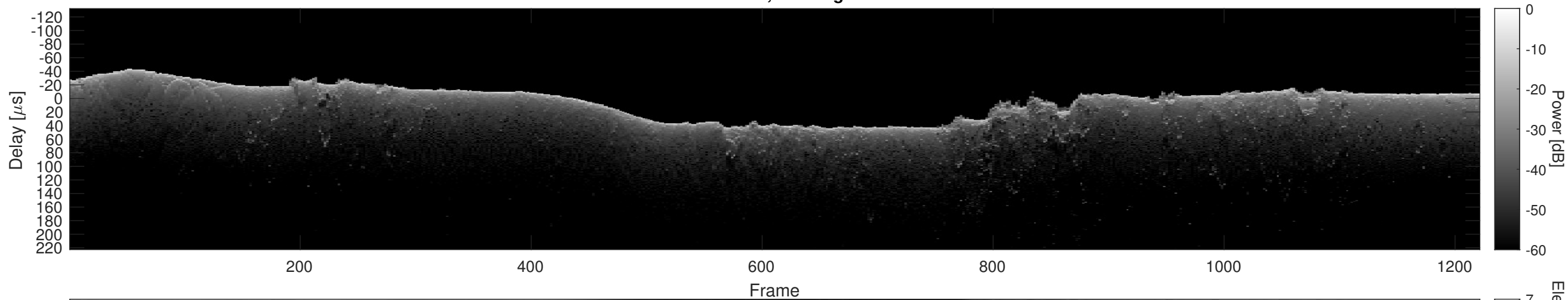
Orbit 23132, Cluttergram
