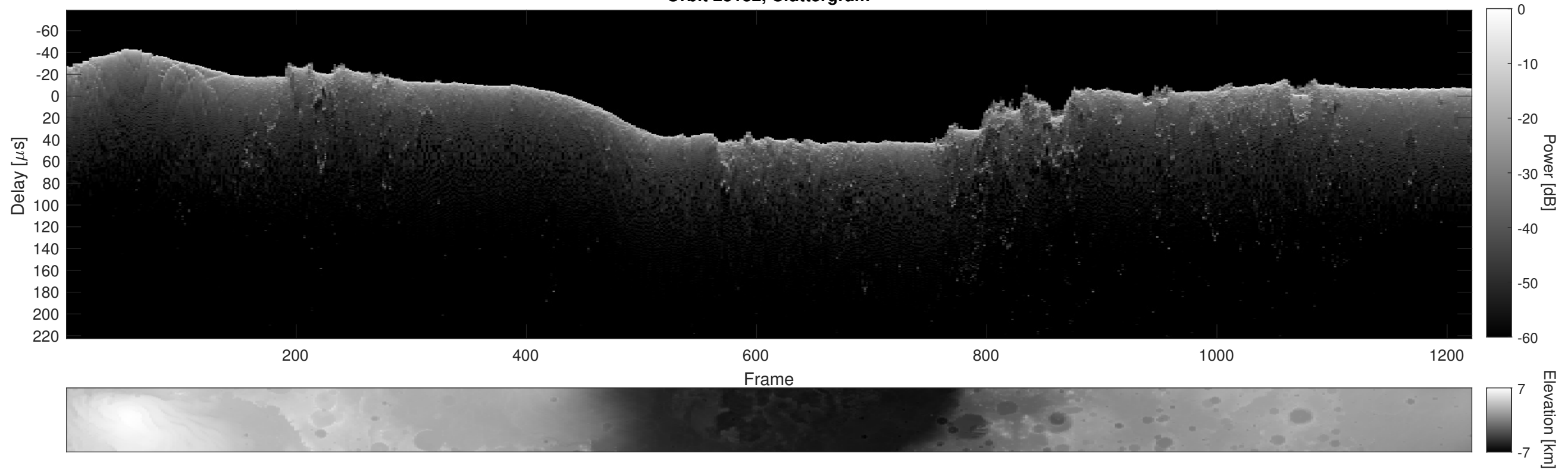
Orbit 23132, Cluttergram
