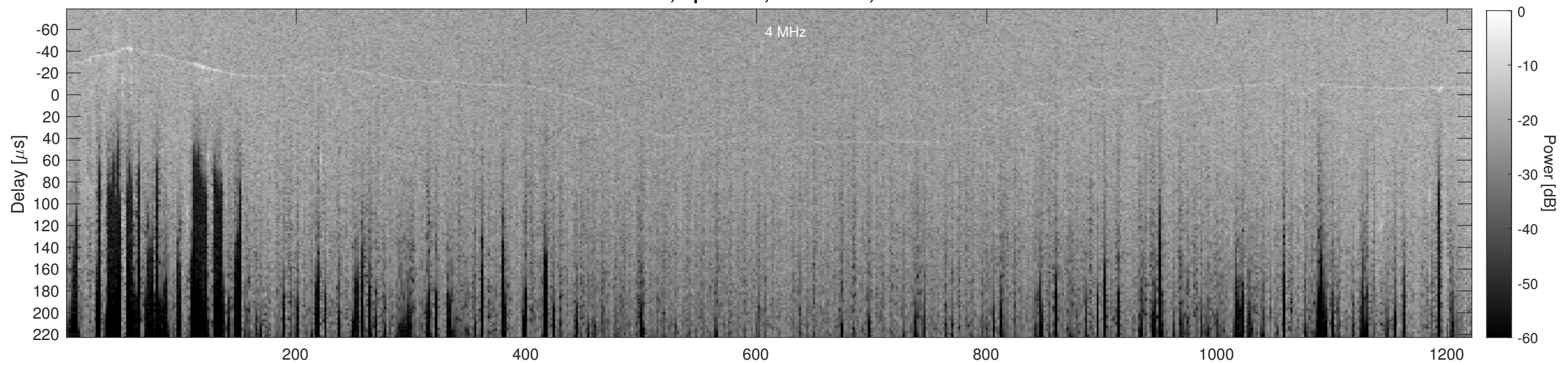
Orbit 23132, Cluttergram
