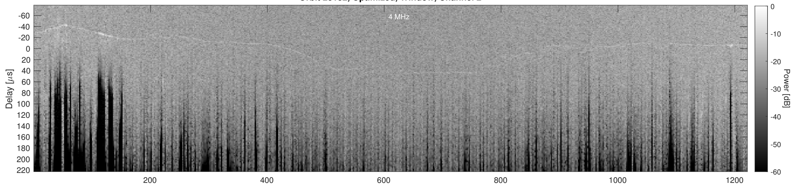
Orbit 23132, Cluttergram
