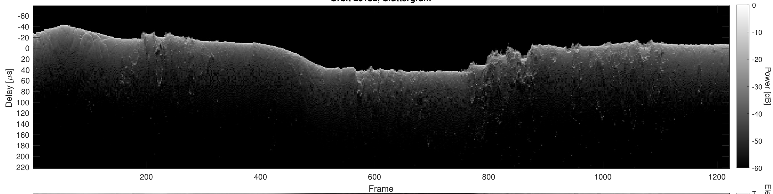
Orbit 23132, Cluttergram
