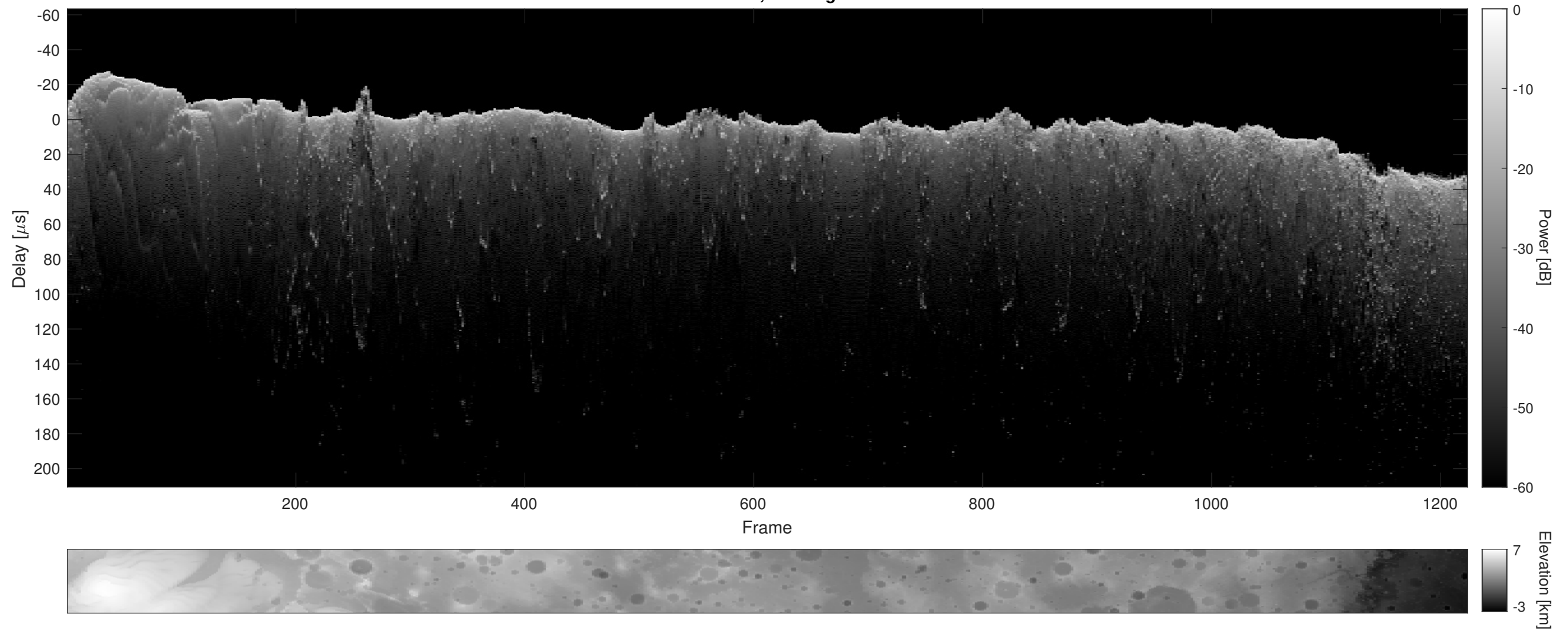
Orbit 23135, Cluttergram
