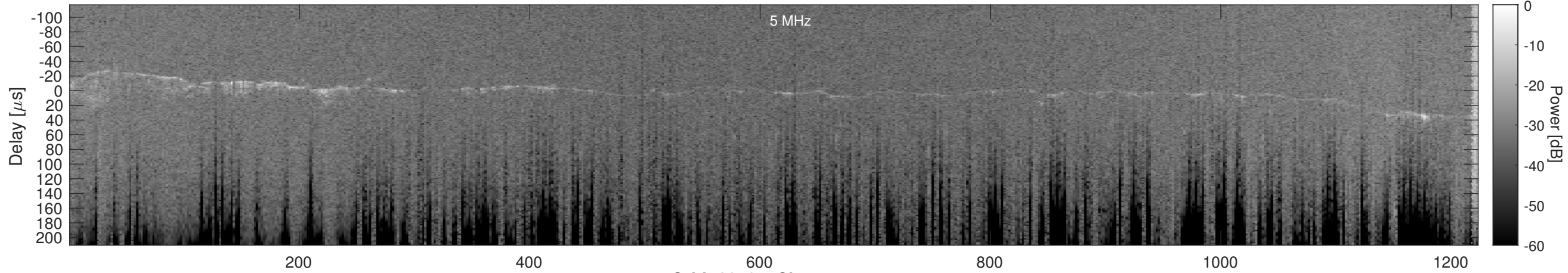
Orbit 23135, Cluttergram
