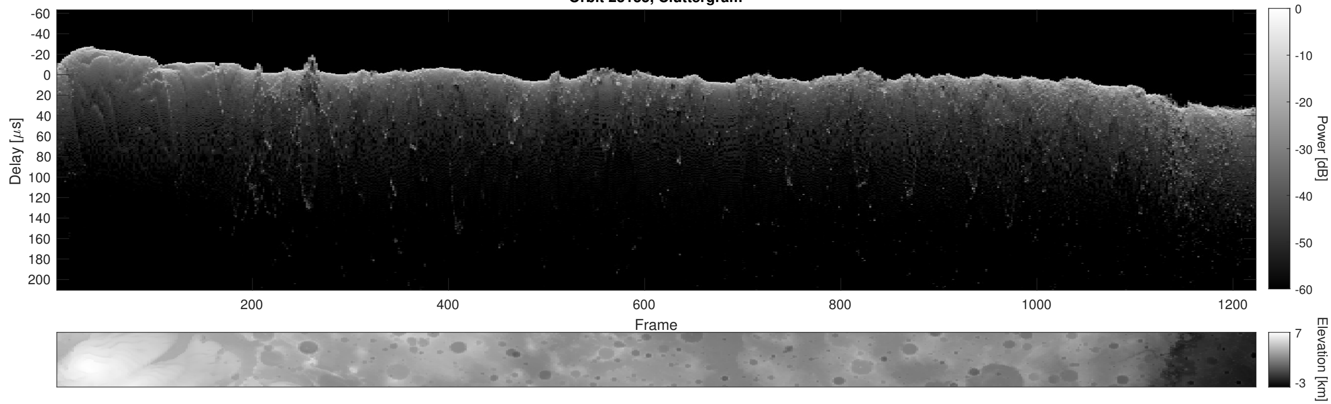
Orbit 23135, Cluttergram
