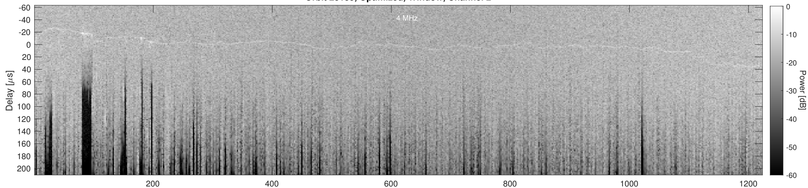
Orbit 23135, Cluttergram
