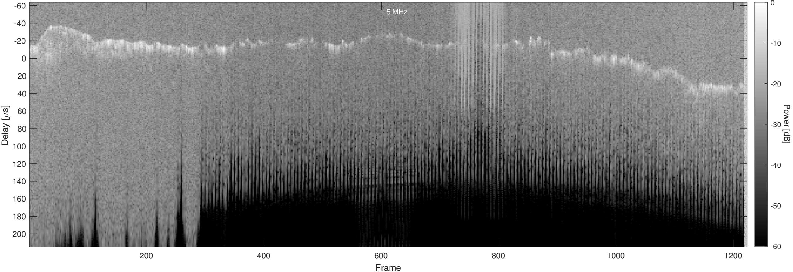
Orbit 23142, Chapman, No Window, Channel 2
