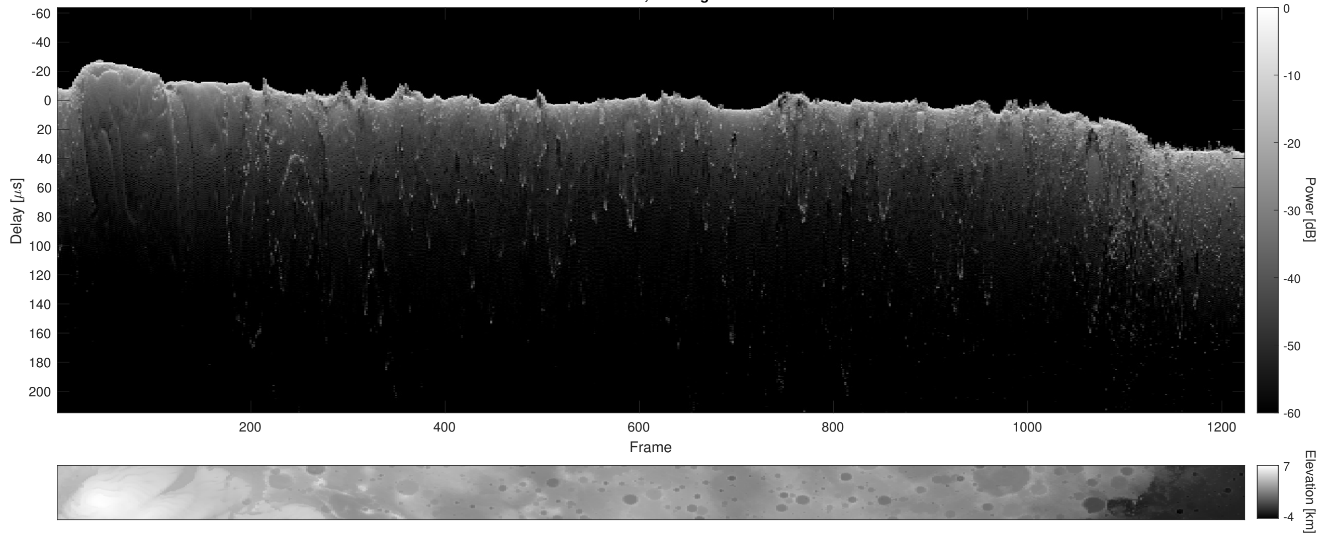
Orbit 23142, Cluttergram
