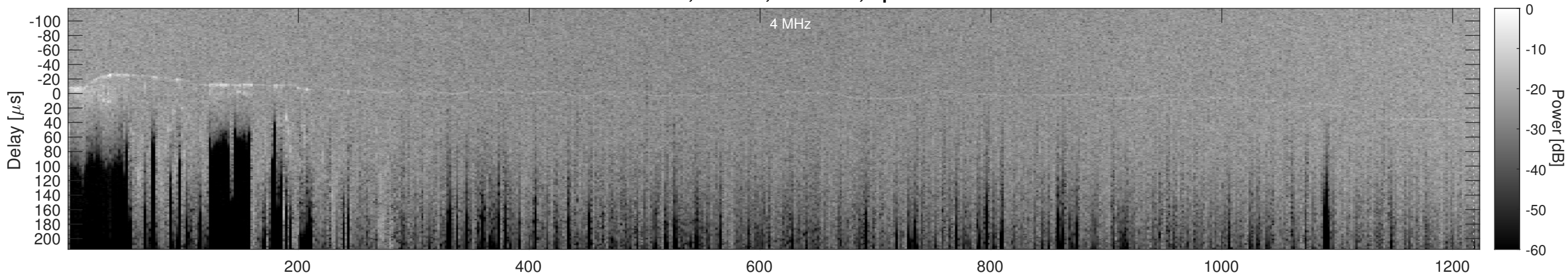
Orbit 23142, Cluttergram
