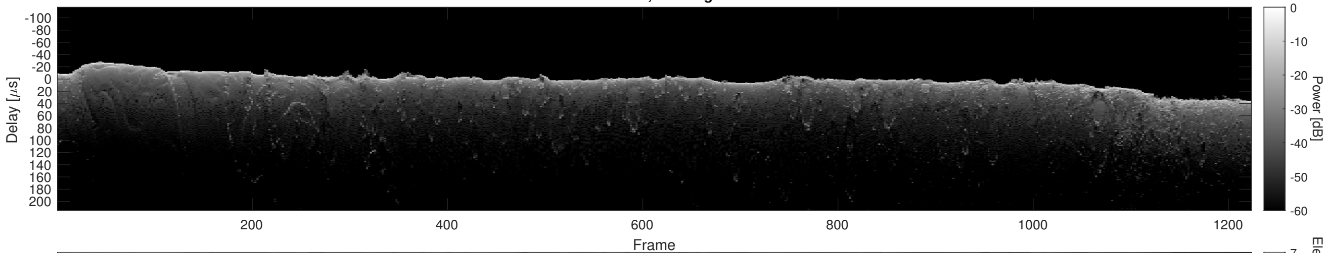
Orbit 23142, Cluttergram
