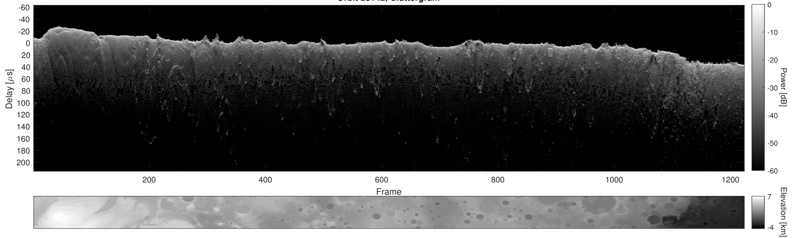
Orbit 23142, Cluttergram
