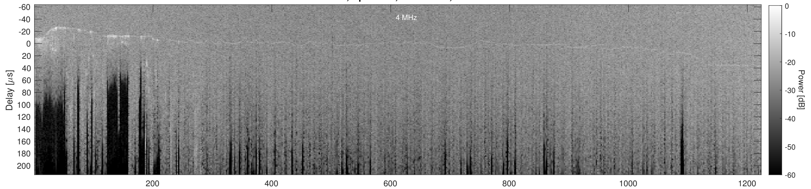
Orbit 23142, Cluttergram
