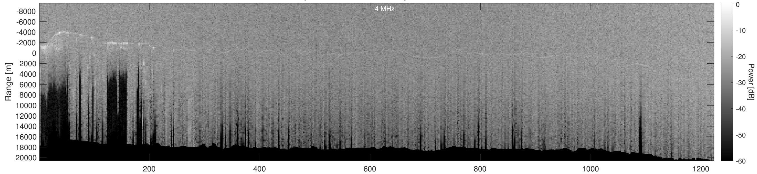
Orbit 23142, Depth-Corrected Cluttergram
