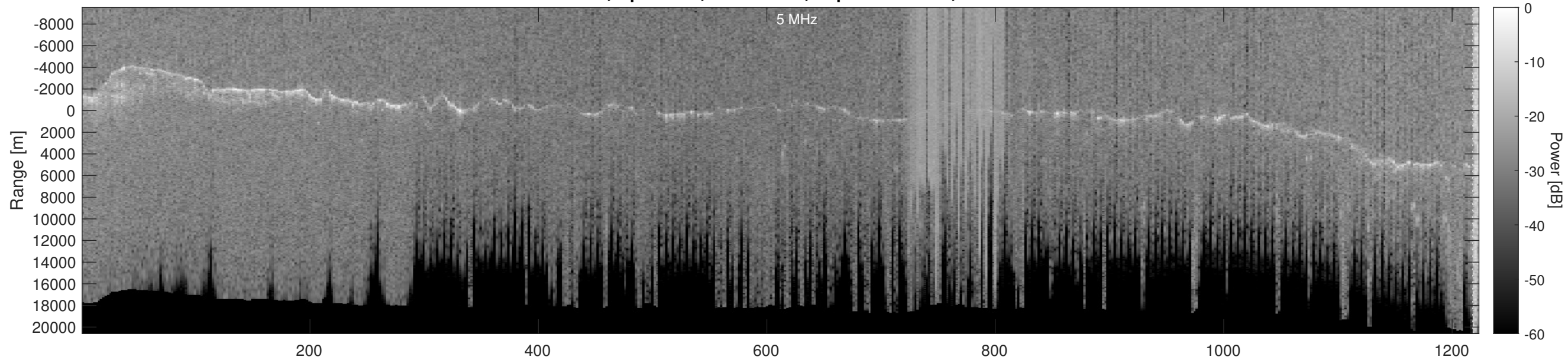
Orbit 23142, Optimized, No Window, Depth-Corrected, Channel 2
