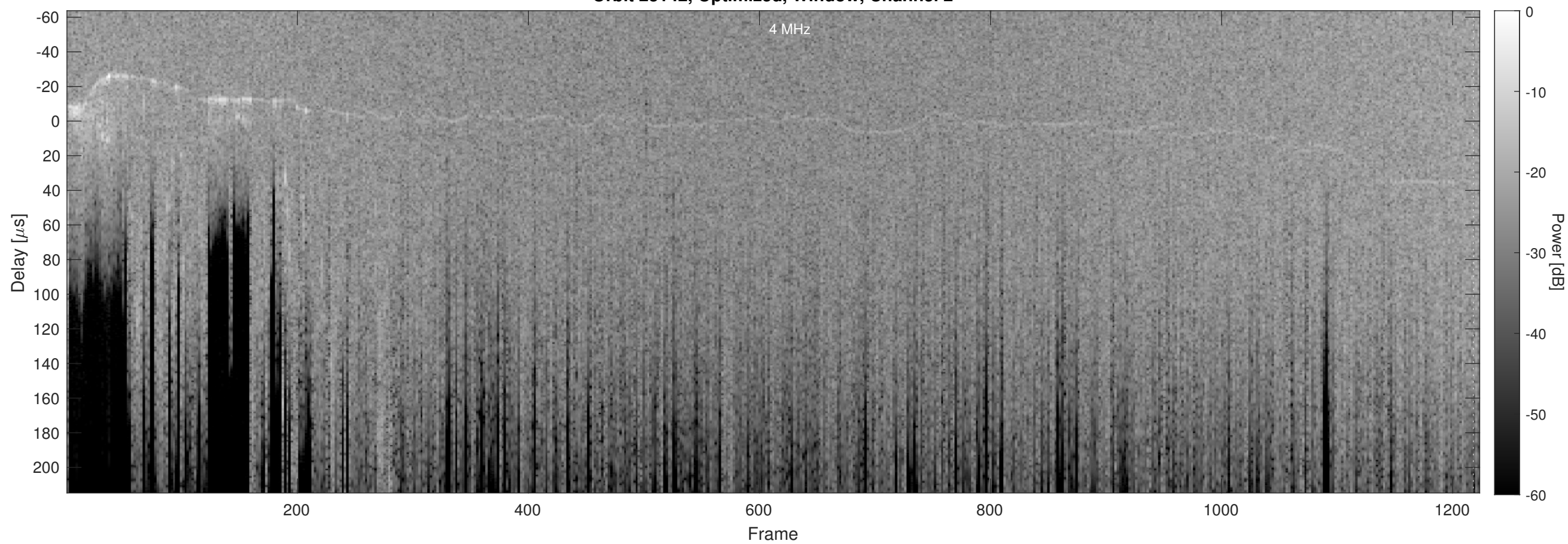
Orbit 23142, Optimized, Window, Channel 2
