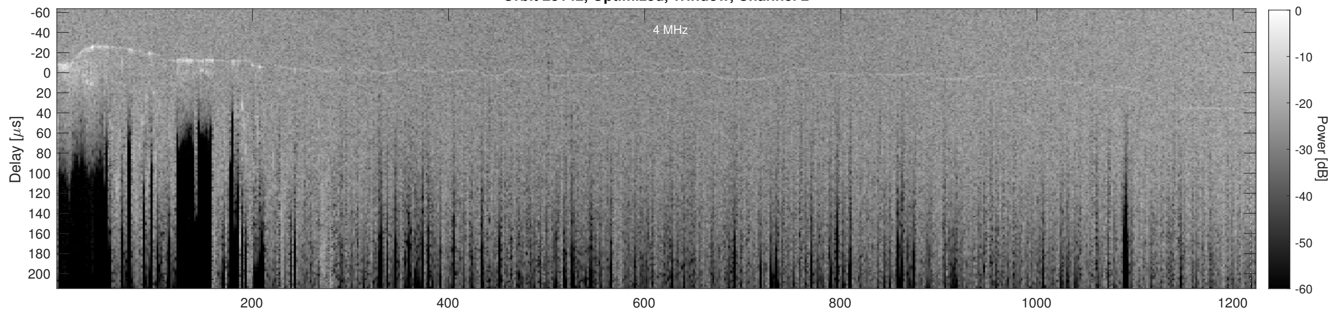
Orbit 23142, Cluttergram
