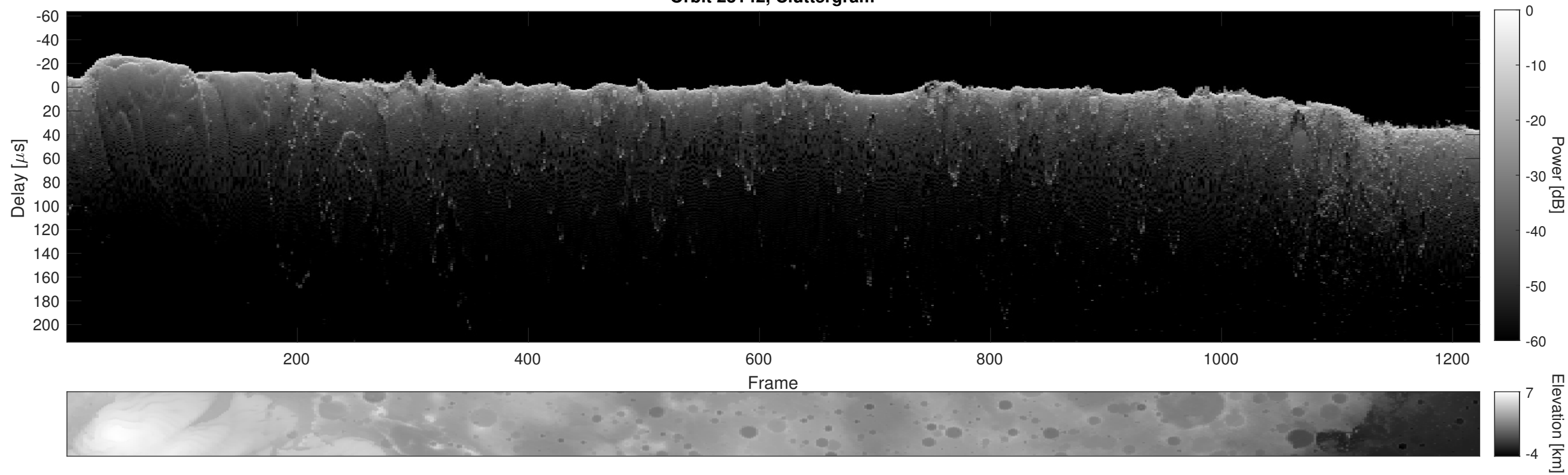
Orbit 23142, Cluttergram
