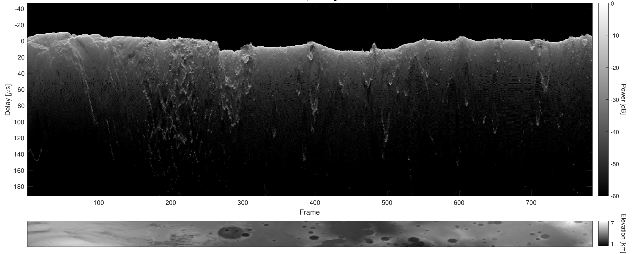
Orbit 23144, Cluttergram
