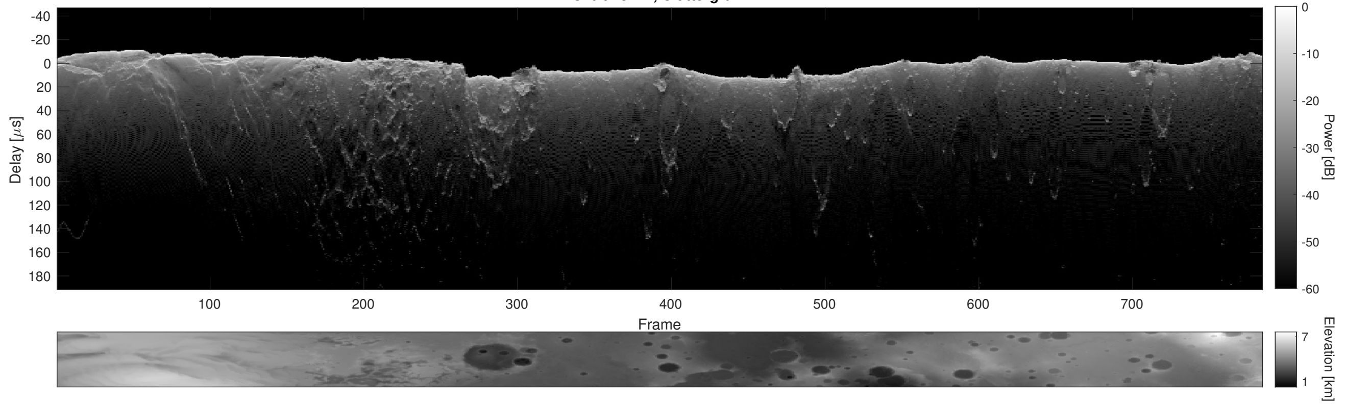
Orbit 23144, Cluttergram
