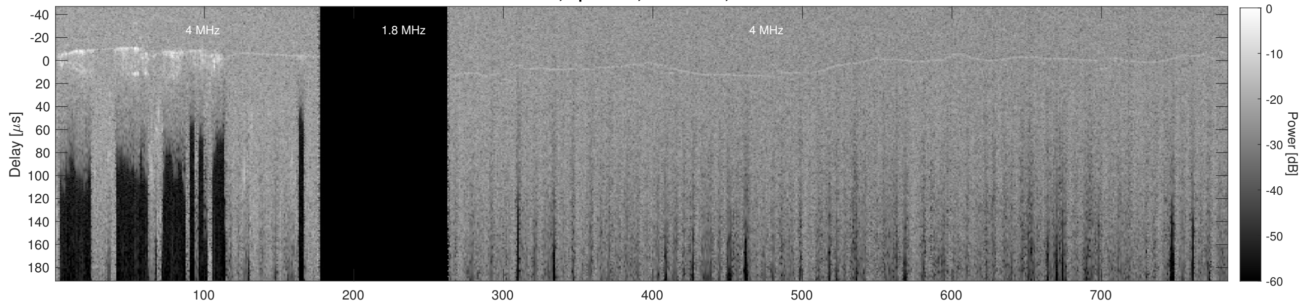
Orbit 23144, Cluttergram
