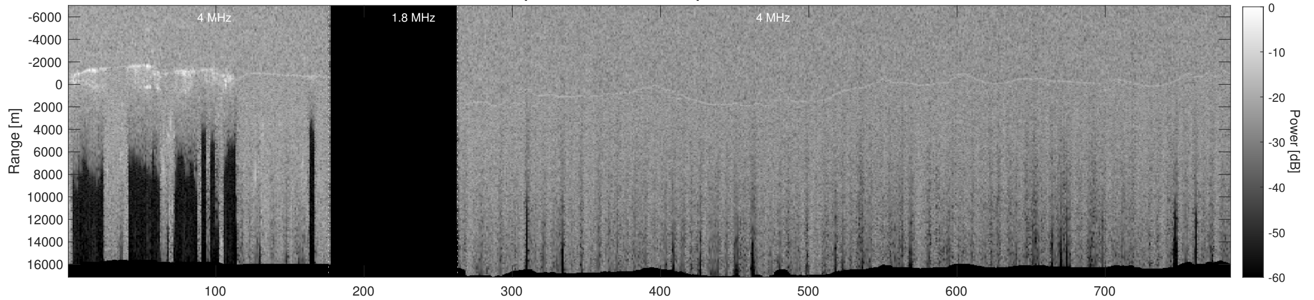
Orbit 23144, Depth-Corrected Cluttergram
