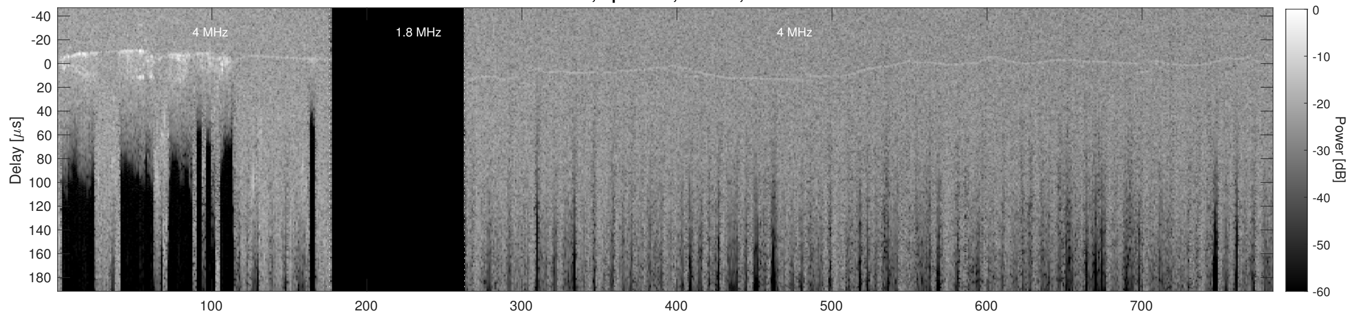
Orbit 23144, Cluttergram
