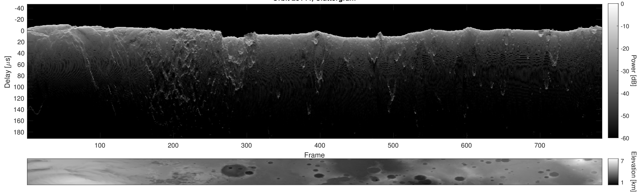
Orbit 23144, Cluttergram
