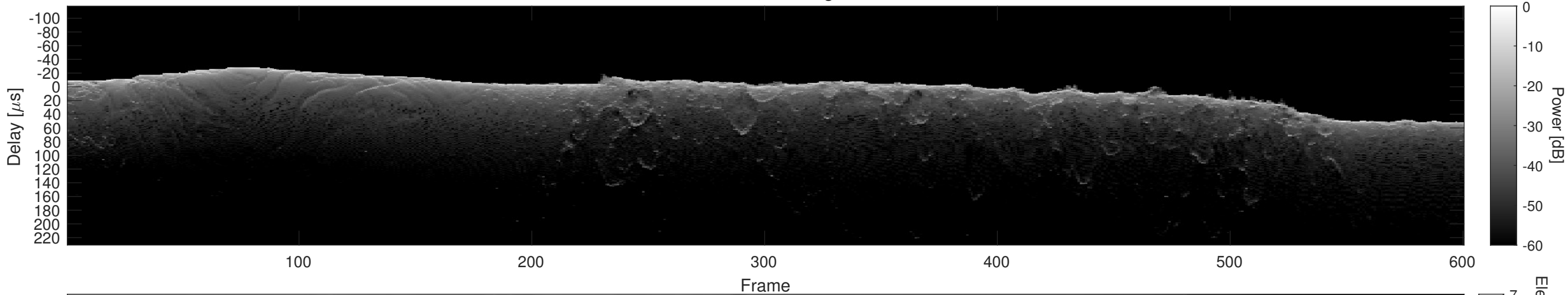
Orbit 23146, Cluttergram
