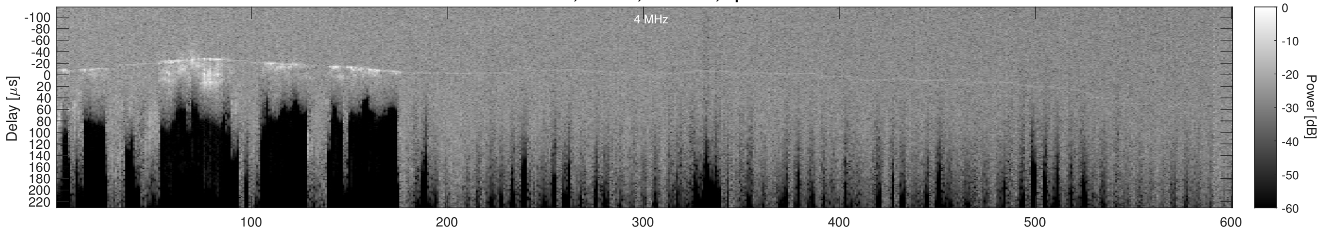
Orbit 23146, Cluttergram
