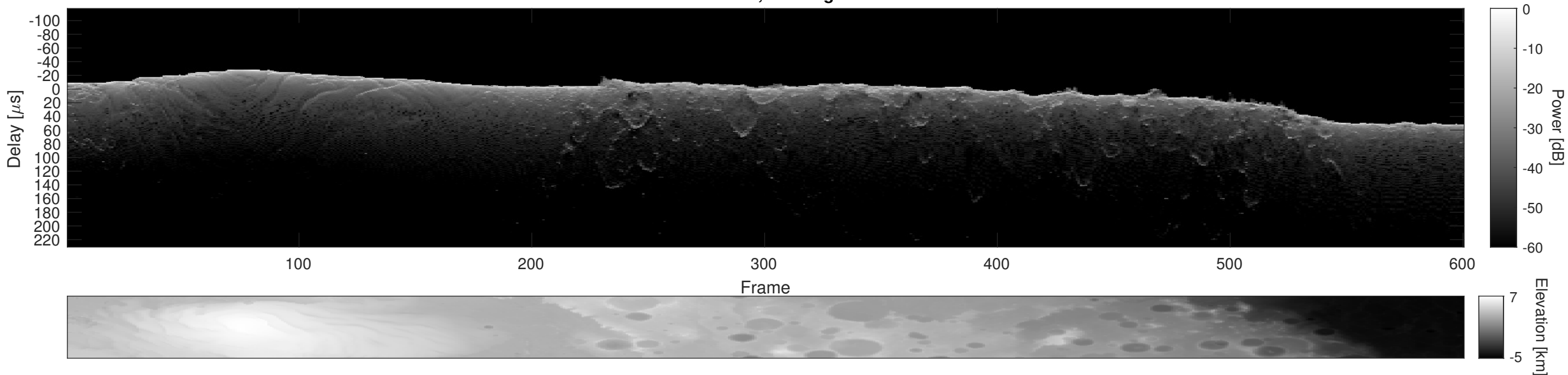
Orbit 23146, Cluttergram
