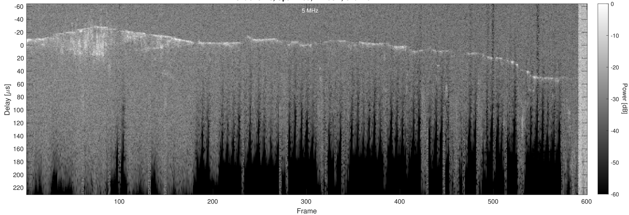
Orbit 23146, Optimized, Window, Channel 2
