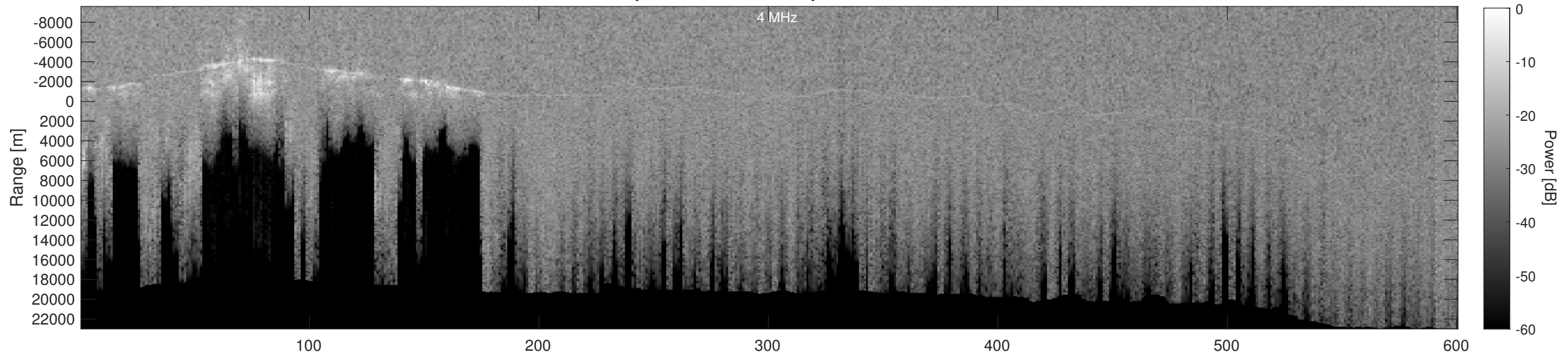
Orbit 23146, Depth-Corrected Cluttergram
