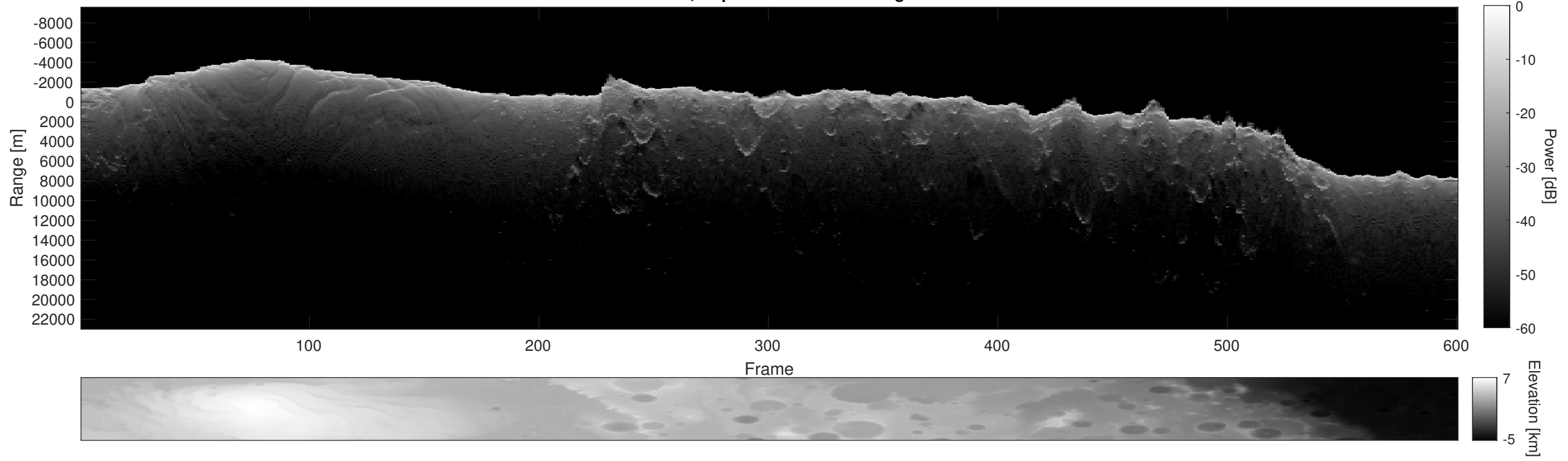
Orbit 23146, Depth-Corrected Cluttergram
