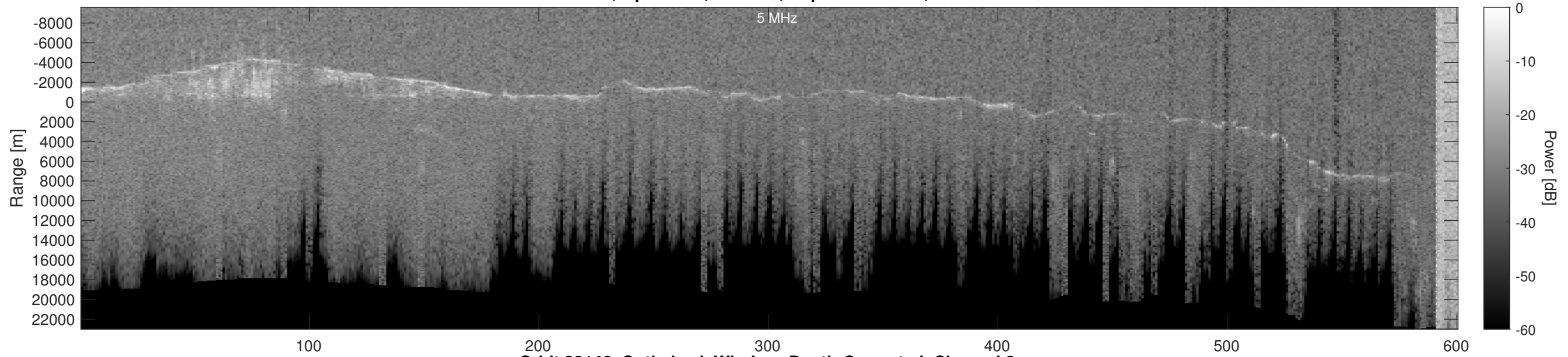
Orbit 23146, Optimized, Window, Depth-Corrected, Channel 2
