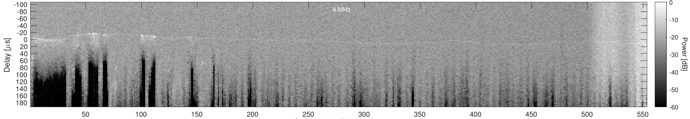
Orbit 23149, Cluttergram
