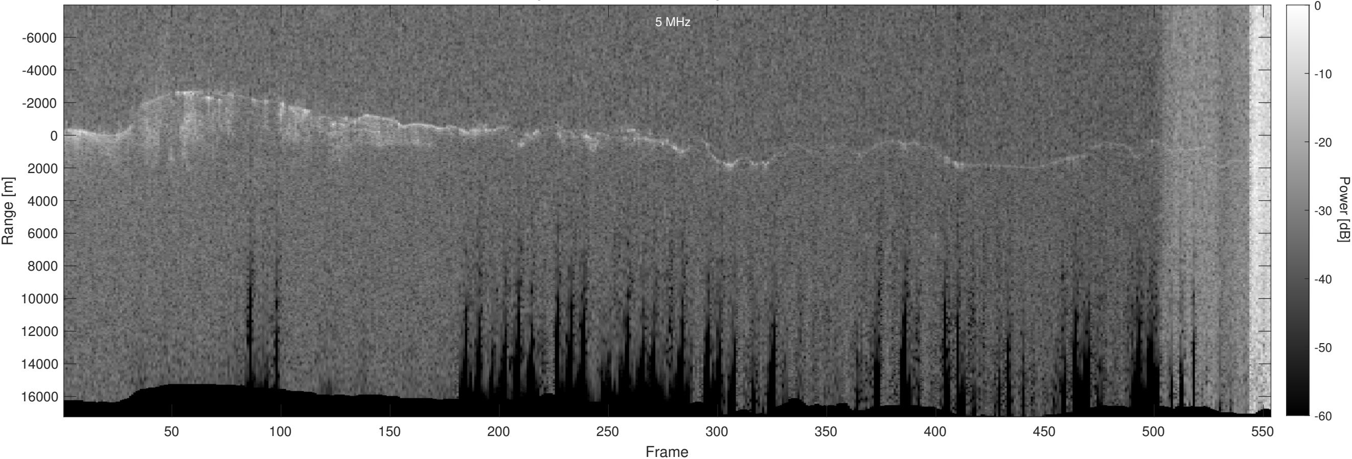
Orbit 23149, Optimized, No Window, Depth-Corrected, Channel 2
