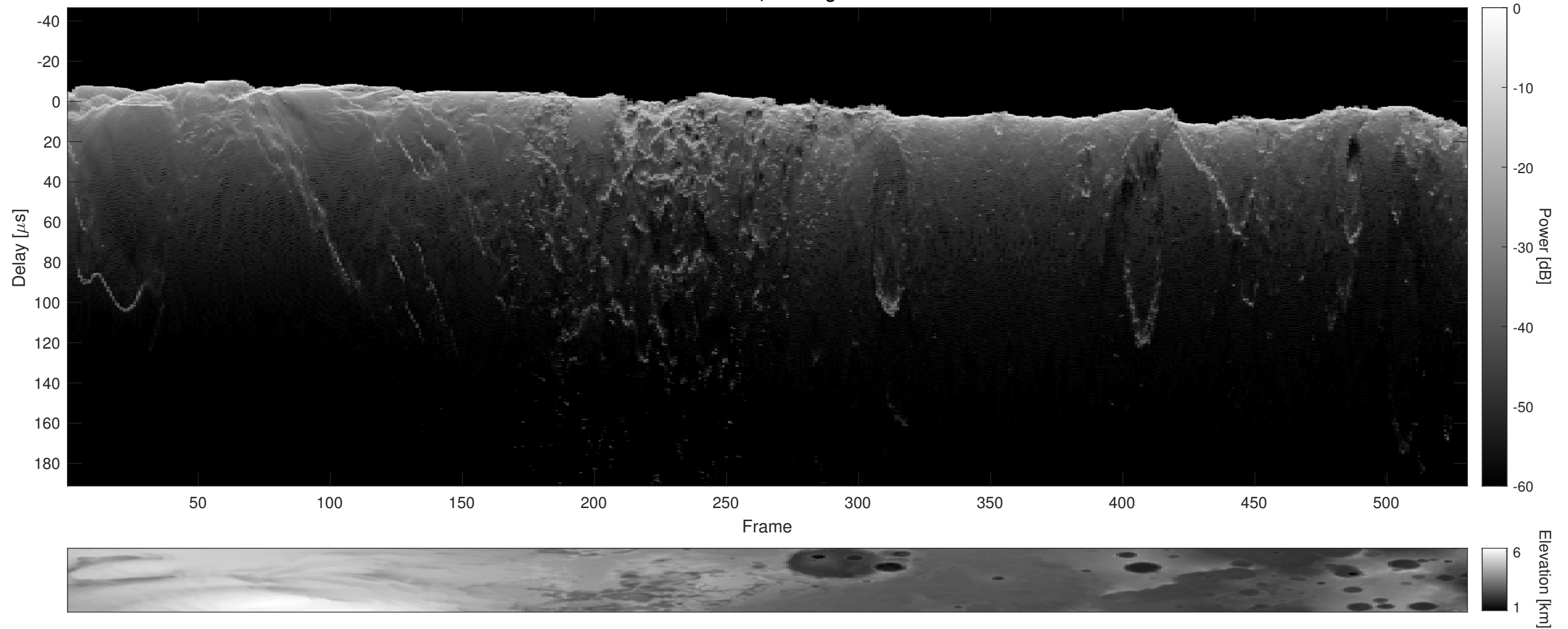
Orbit 23151, Cluttergram
