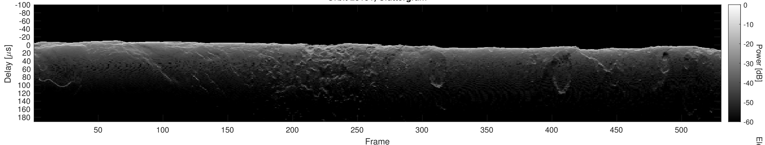
Orbit 23151, Cluttergram
