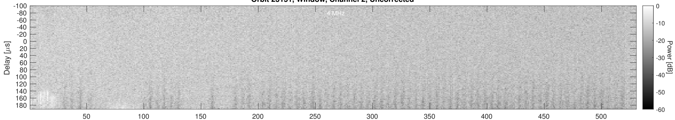
Orbit 23151, Window, Channel 2, Chapman
