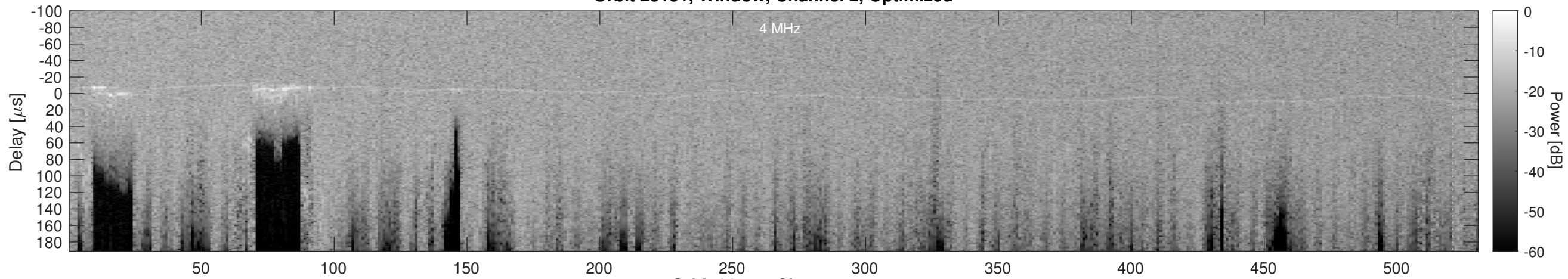
Orbit 23151, Cluttergram
