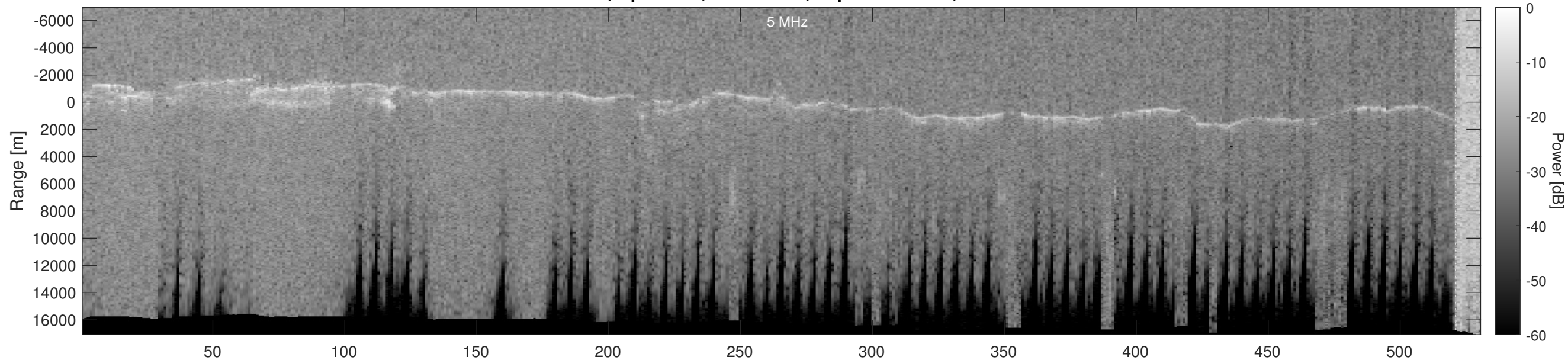
Orbit 23151, Optimized, No Window, Depth-Corrected, Channel 2
