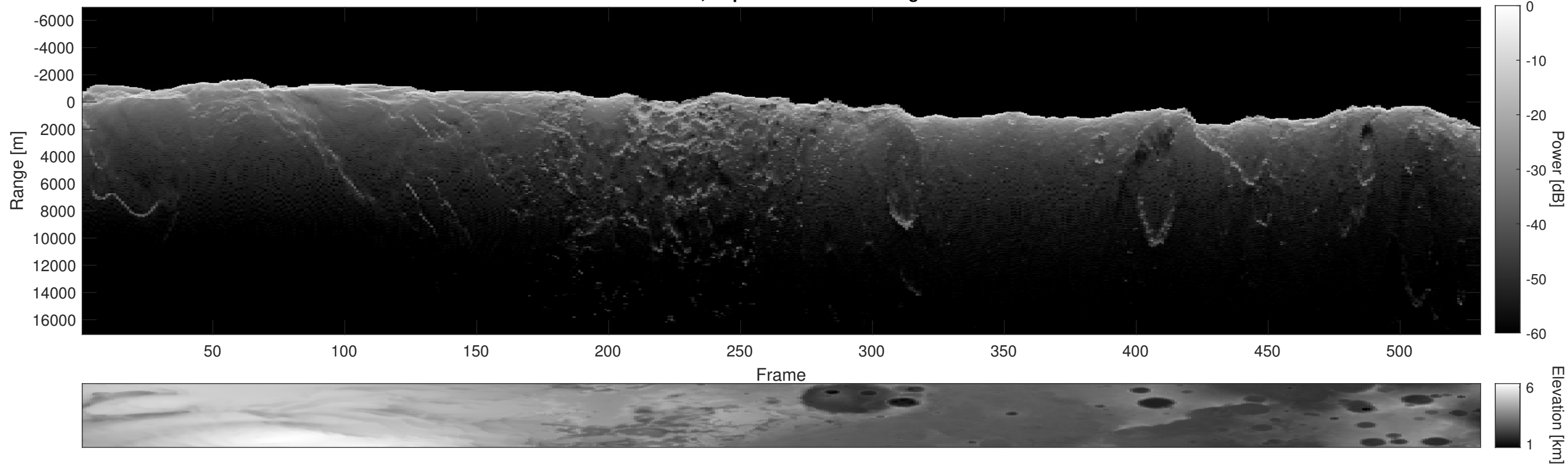
Orbit 23151, Depth-Corrected Cluttergram
