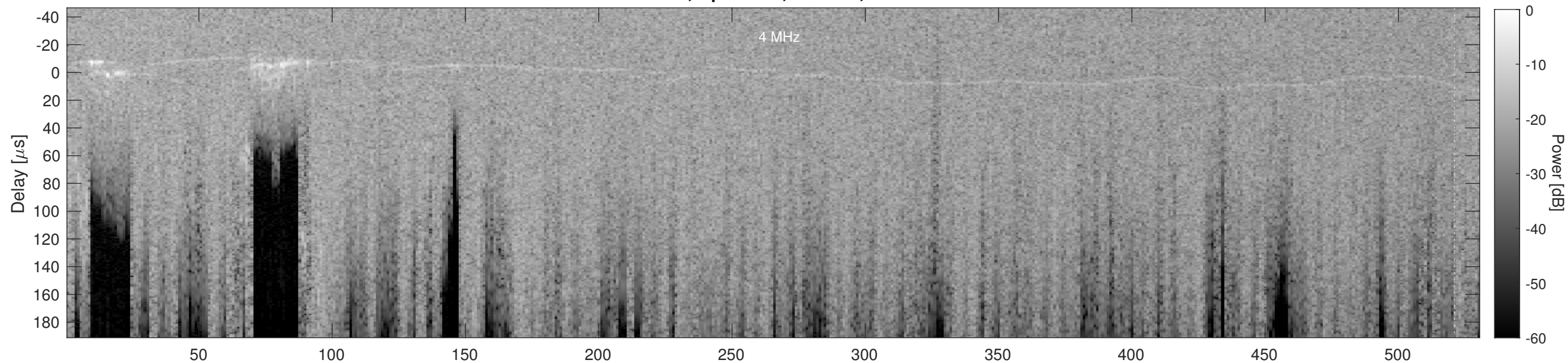
Orbit 23151, Cluttergram
