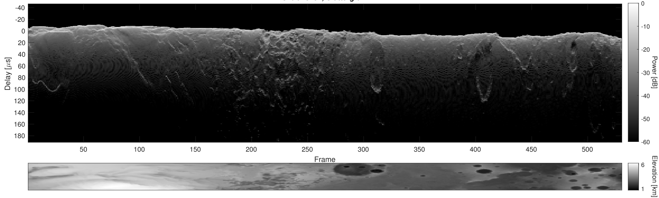
Orbit 23151, Cluttergram
