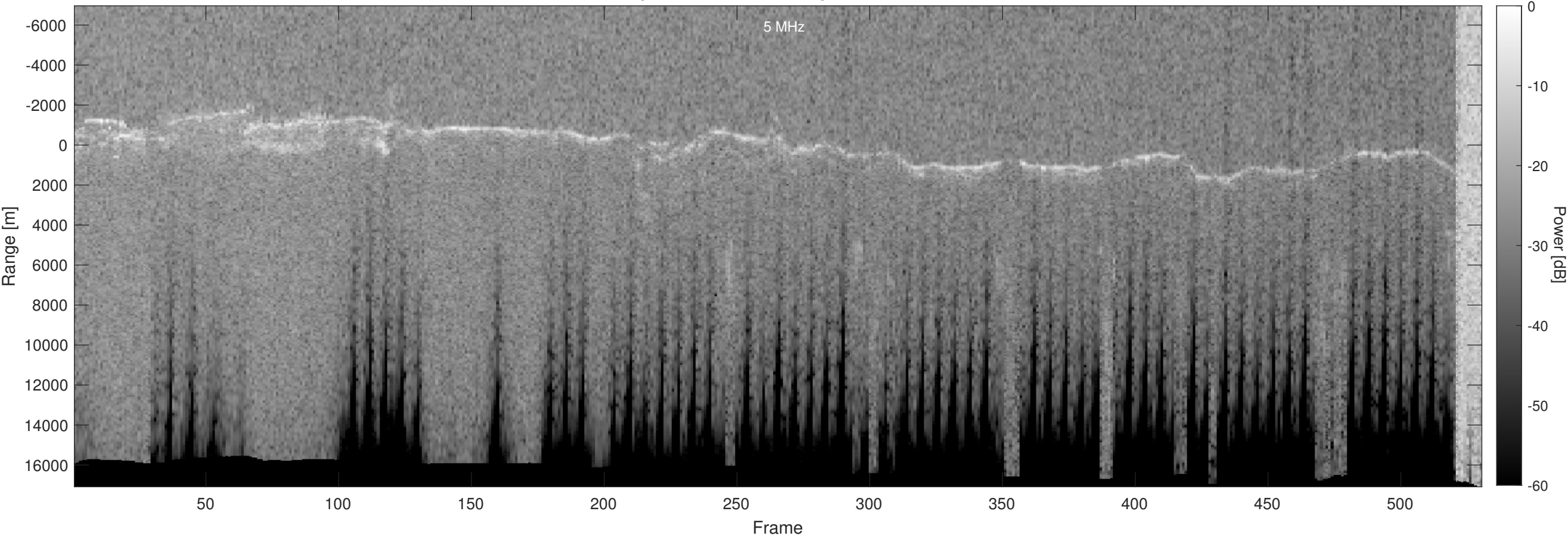
Orbit 23151, Optimized, Window, Depth-Corrected, Channel 2
