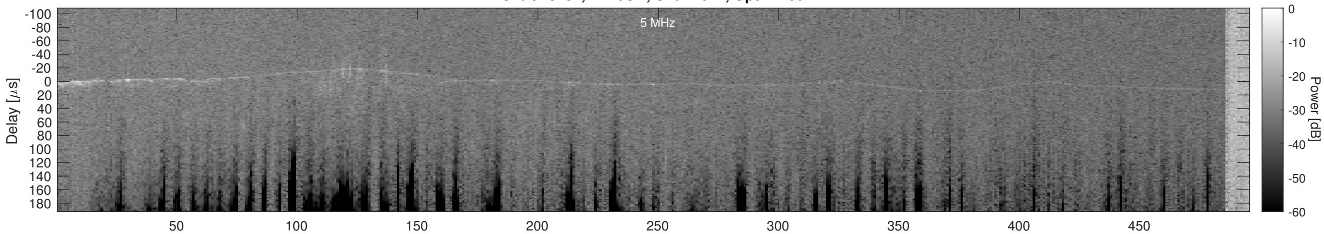
Orbit 23157, Cluttergram
