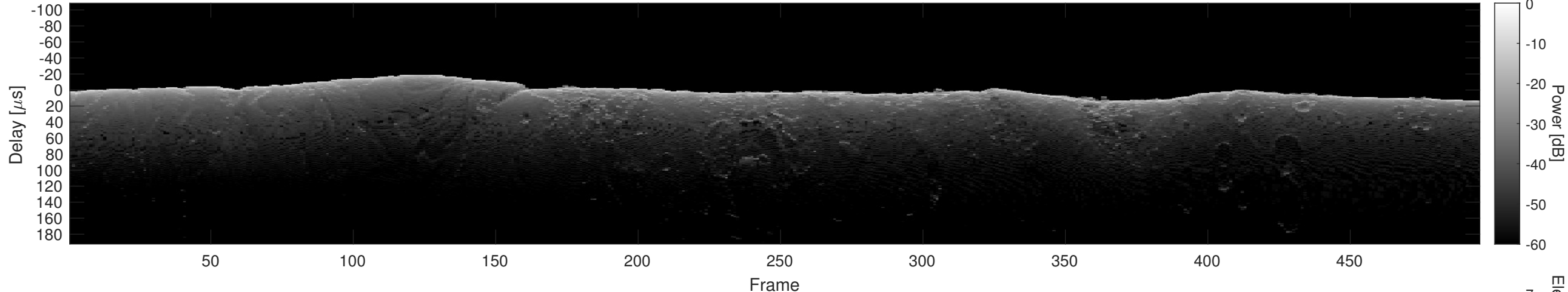
Orbit 23157, Cluttergram
