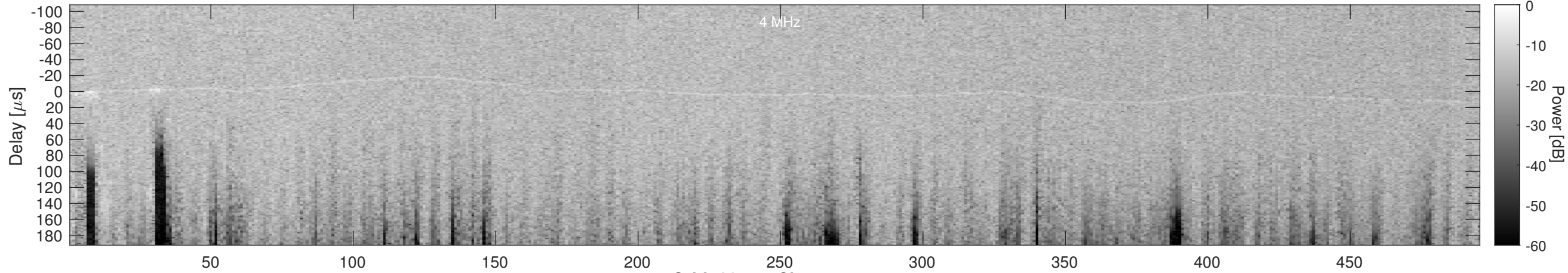
Orbit 23157, Cluttergram
