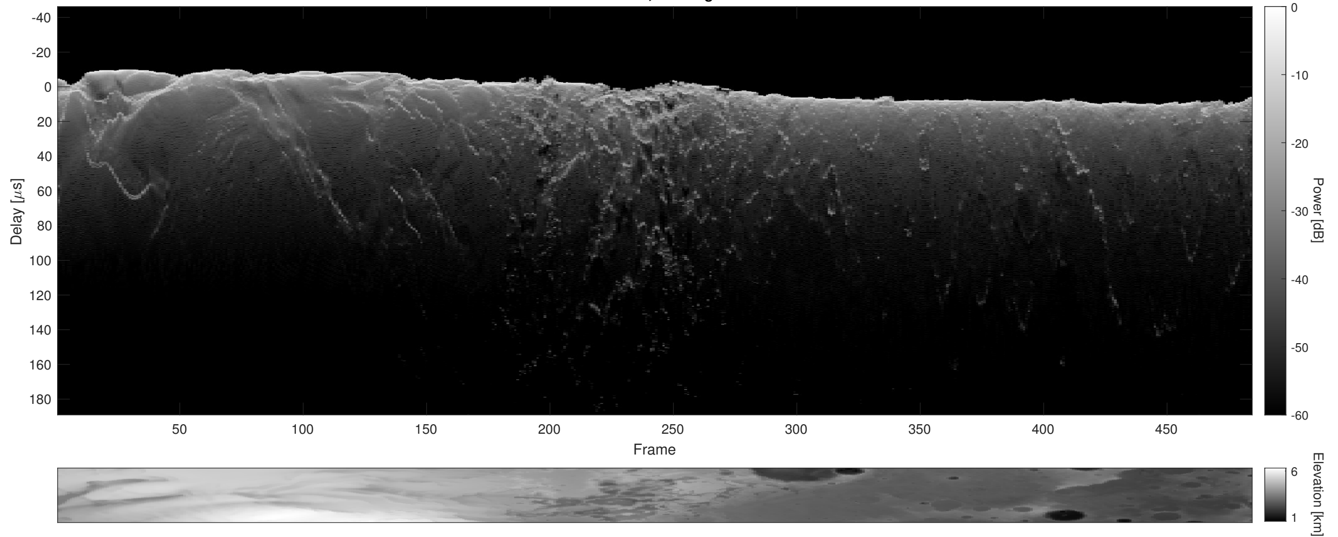
Orbit 23158, Cluttergram
