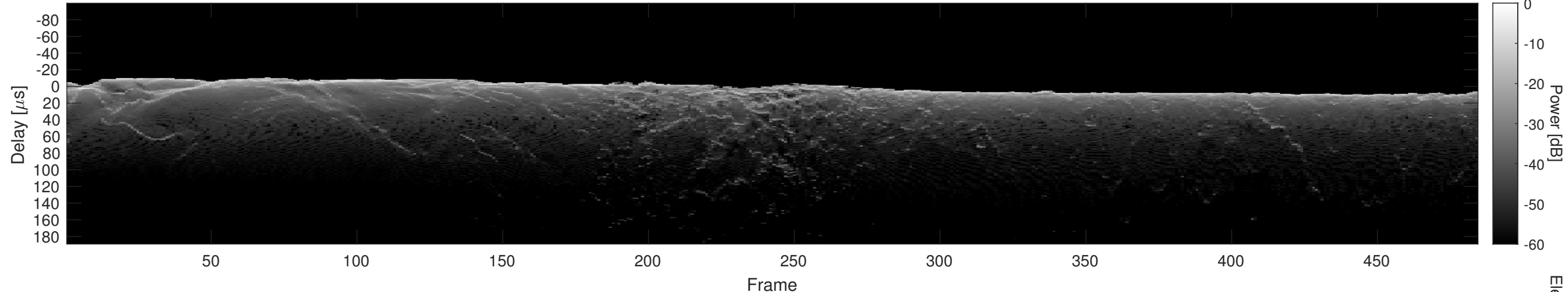
Orbit 23158, Cluttergram
