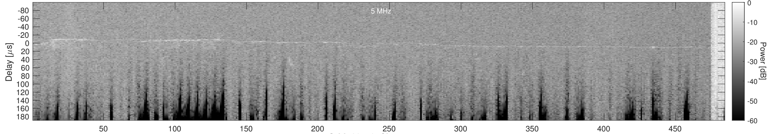
Orbit 23158, Cluttergram
