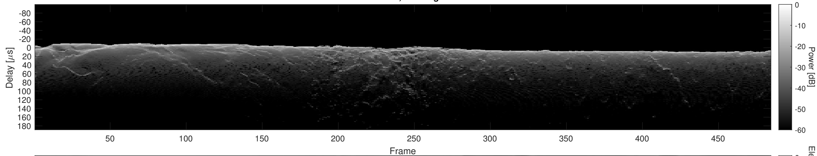
Orbit 23158, Cluttergram
