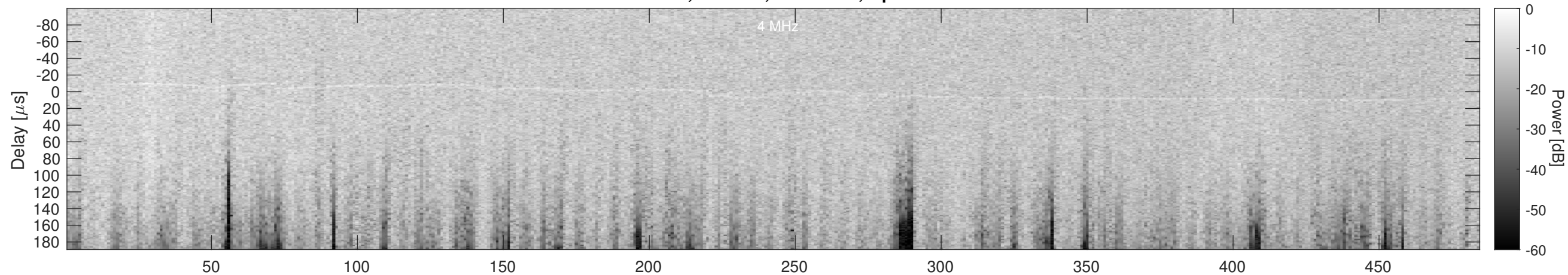
Orbit 23158, Cluttergram
