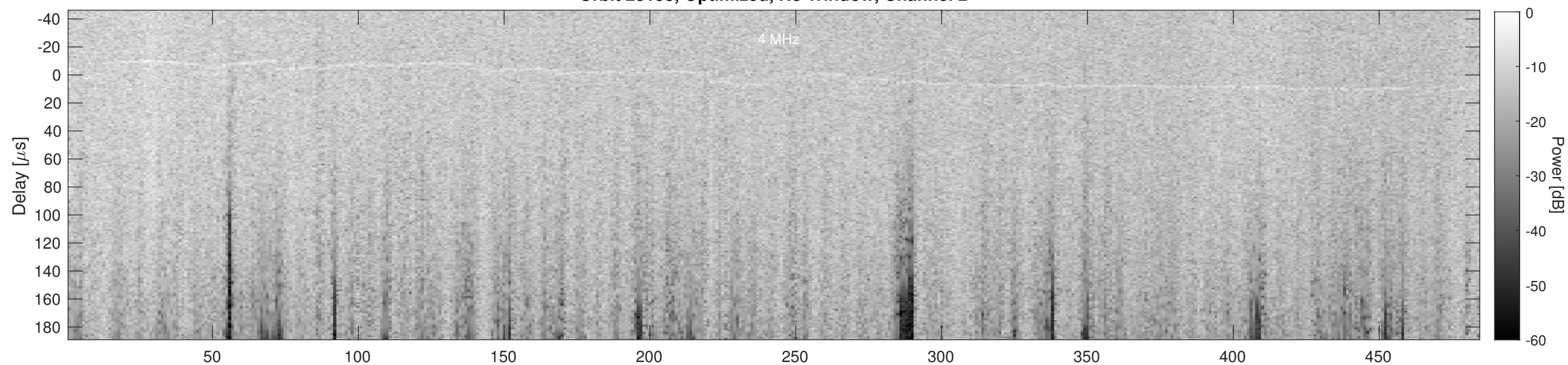
Orbit 23158, Cluttergram
