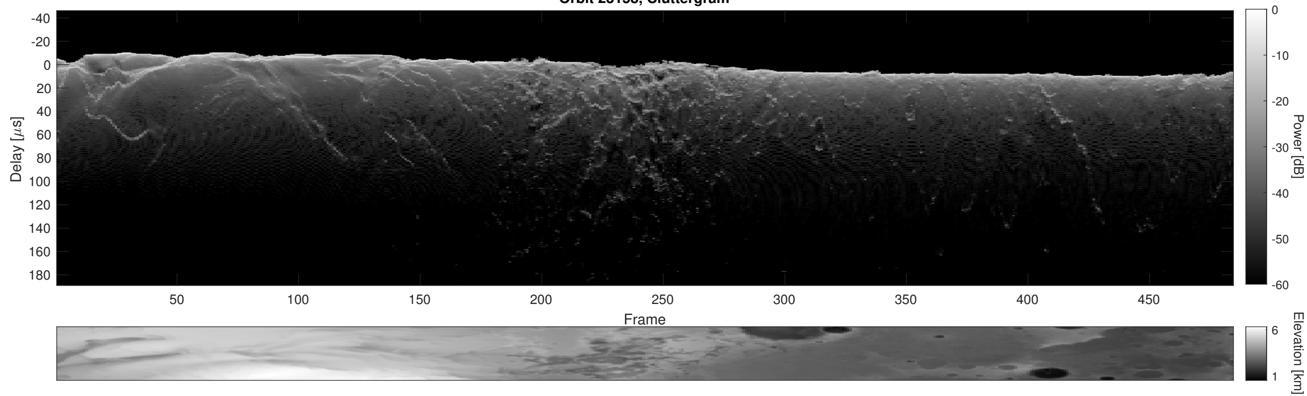
Orbit 23158, Cluttergram
