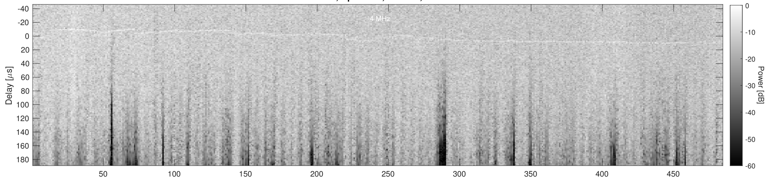
Orbit 23158, Cluttergram
