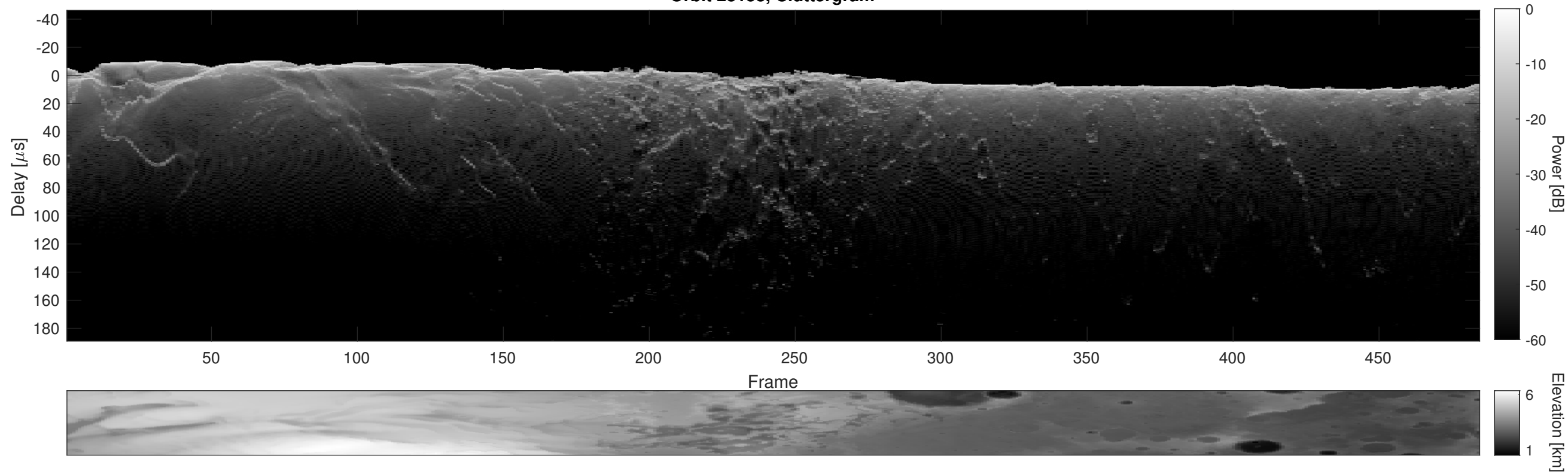
Orbit 23158, Cluttergram
