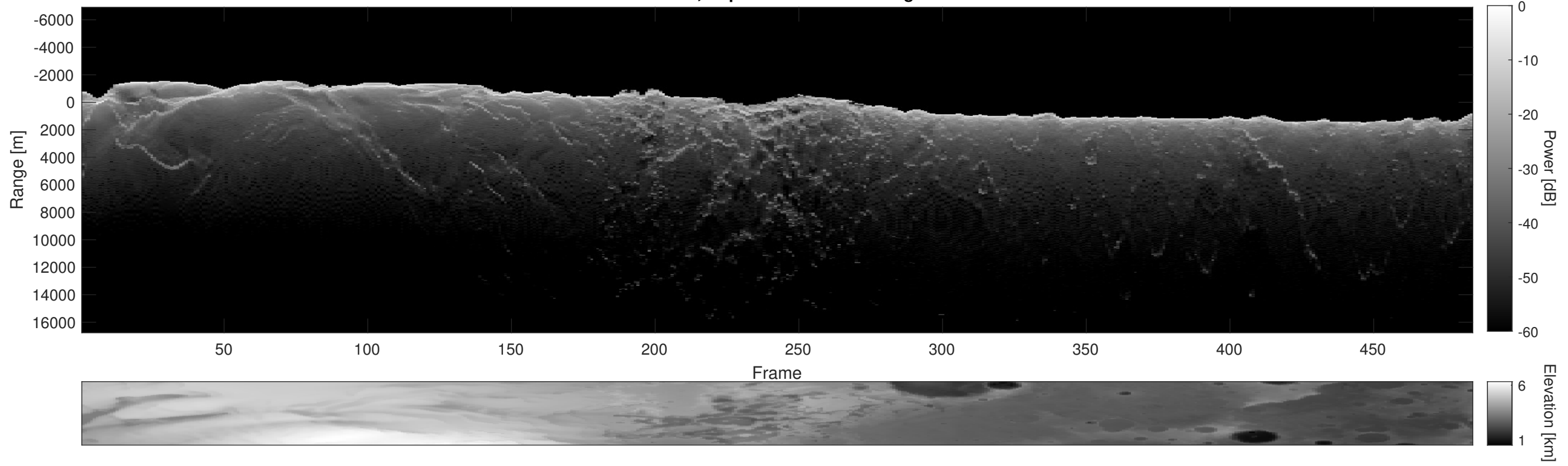
Orbit 23158, Depth-Corrected Cluttergram
