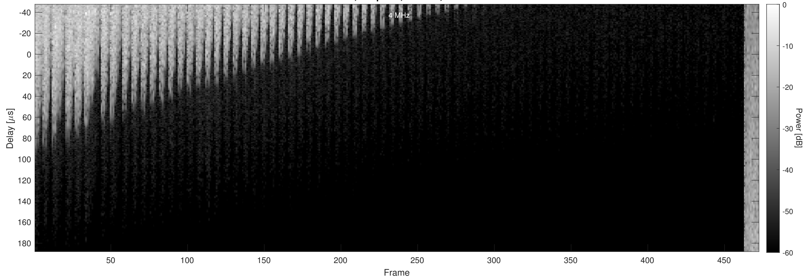
Orbit 23161, Chapman, Window, Channel 2
