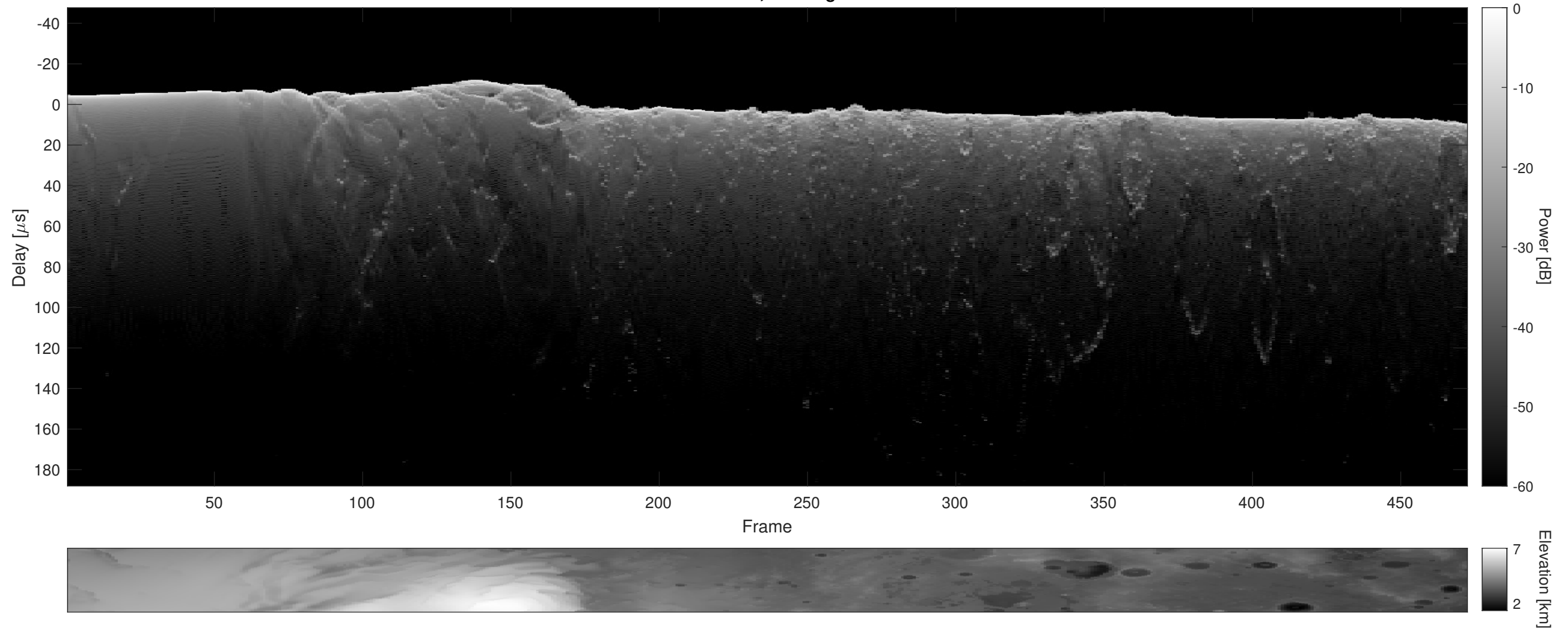
Orbit 23161, Cluttergram
