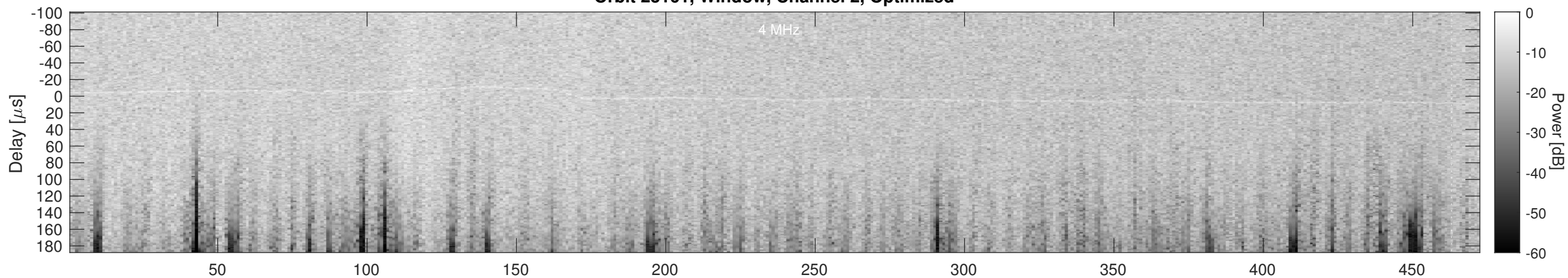
Orbit 23161, Cluttergram
