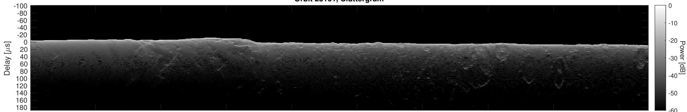
Orbit 23161, Cluttergram
