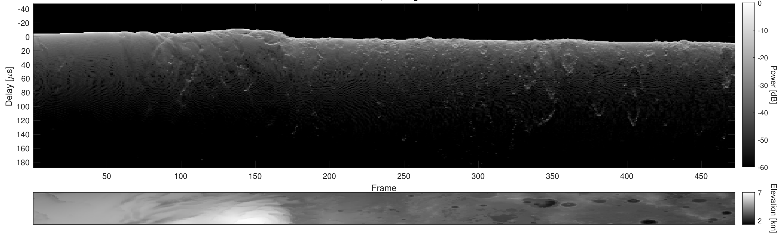
Orbit 23161, Cluttergram
