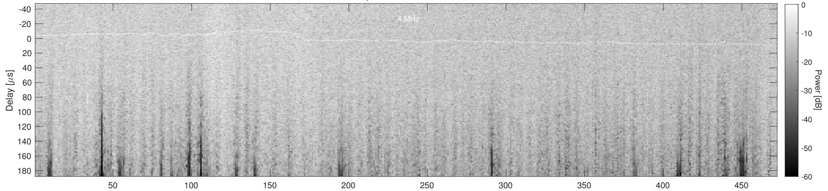
Orbit 23161, Cluttergram
