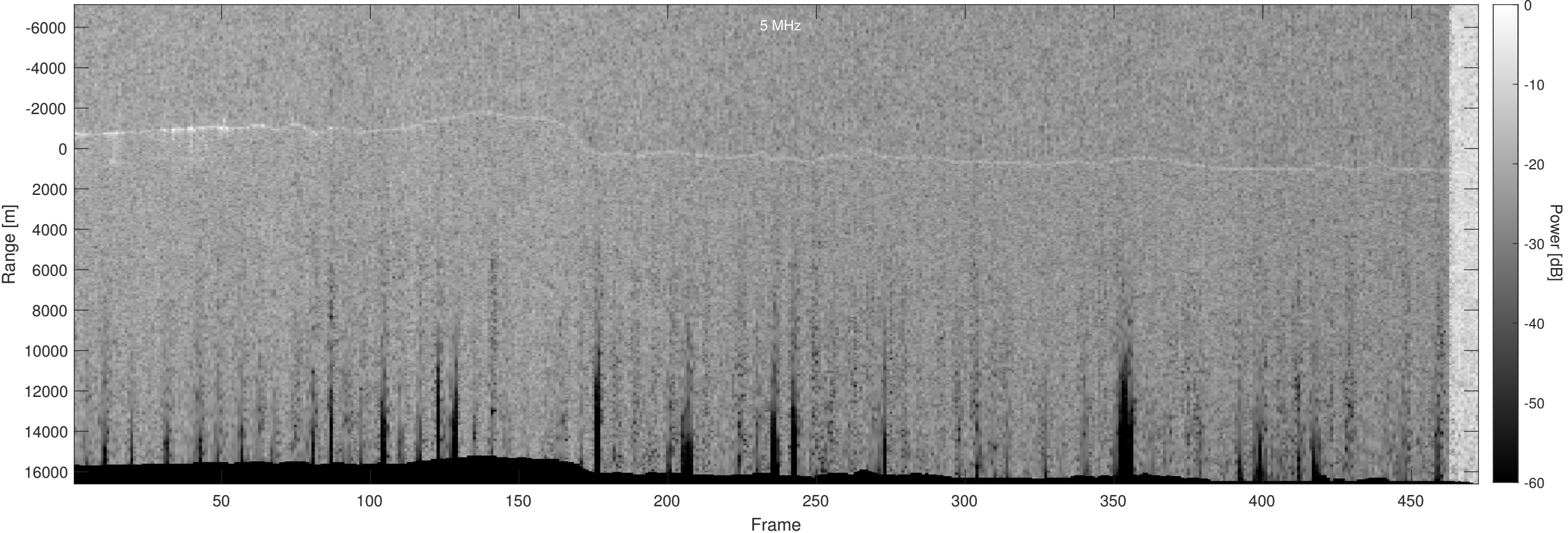
Orbit 23161, Optimized, No Window, Depth-Corrected, Channel 2
