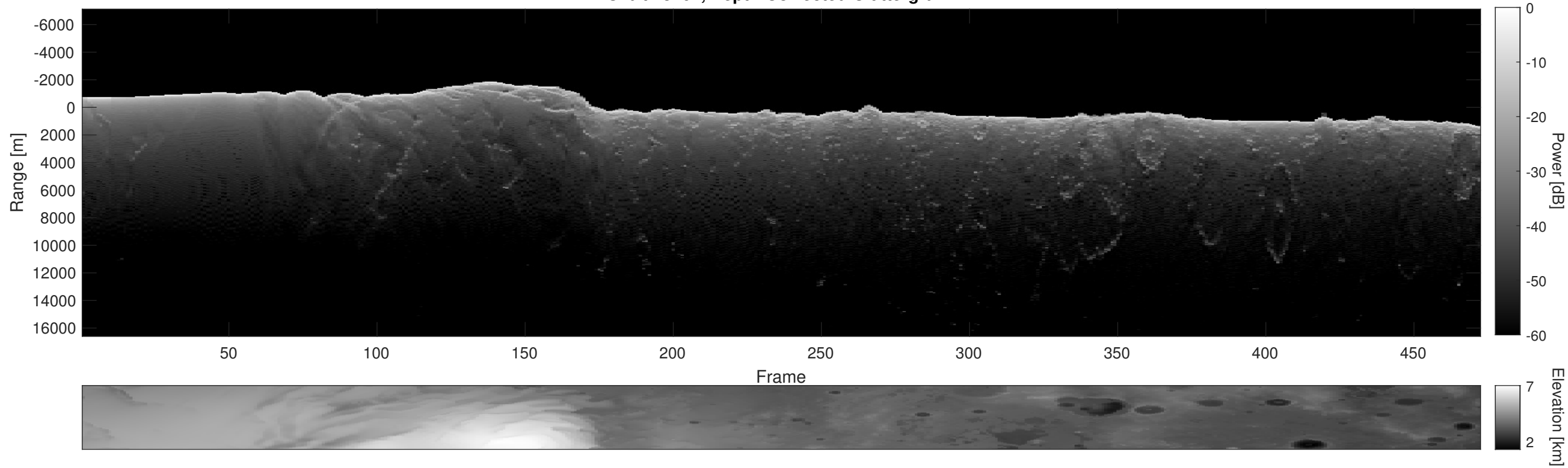
Orbit 23161, Depth-Corrected Cluttergram
