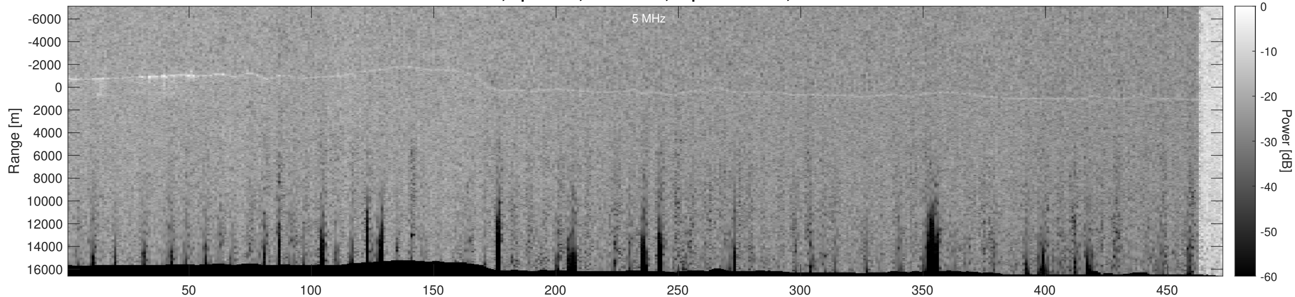
Orbit 23161, Optimized, No Window, Depth-Corrected, Channel 2
