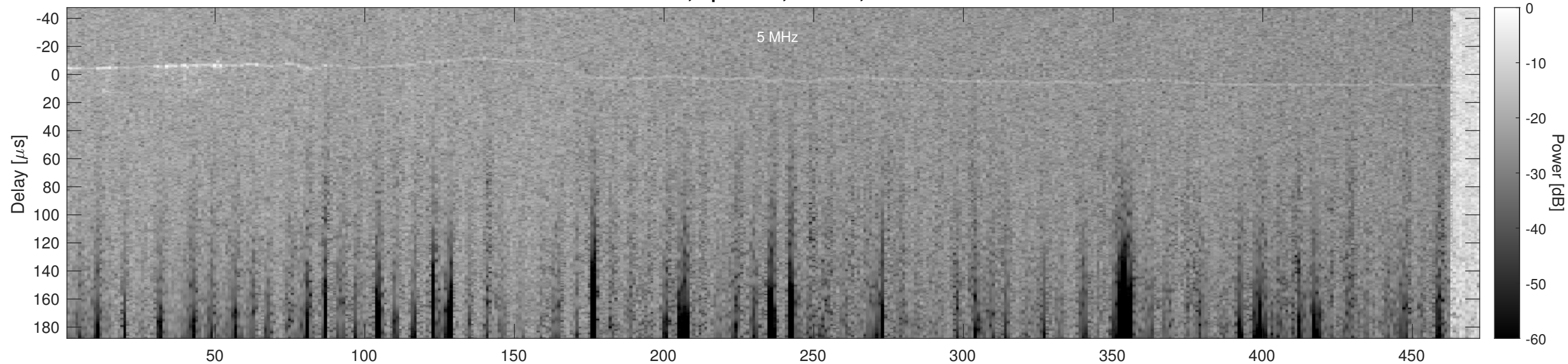
Orbit 23161, Optimized, Window, Channel 2
