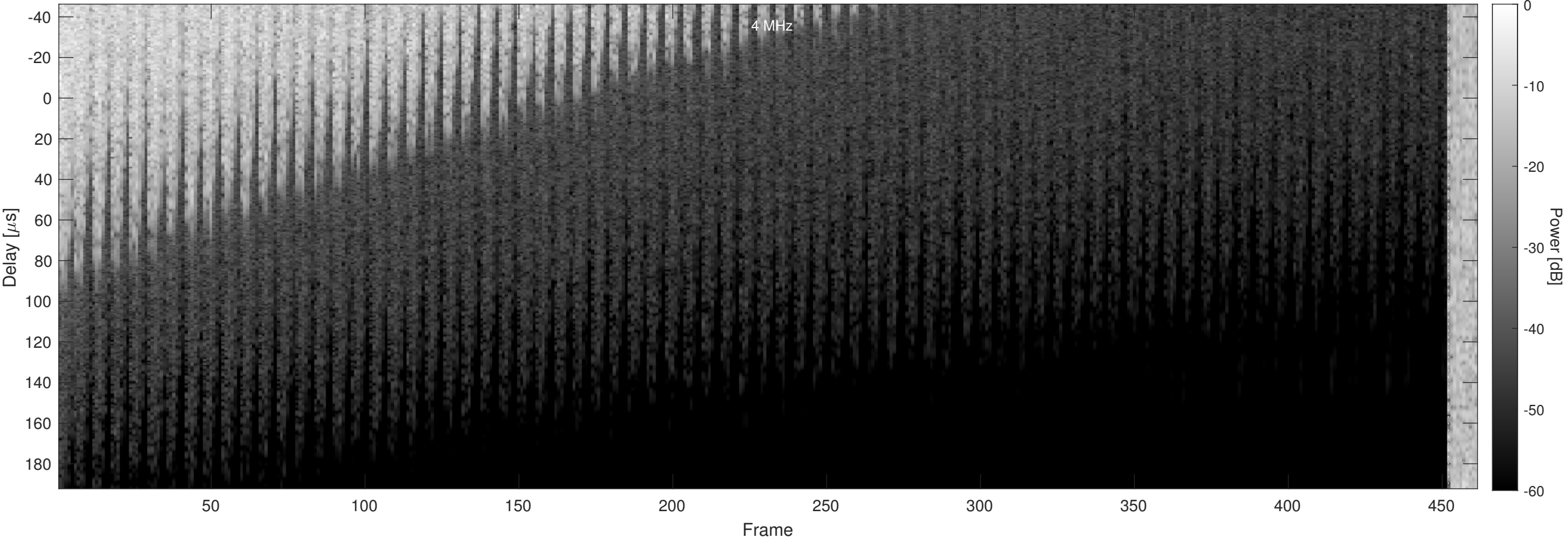
Orbit 23165, Chapman, No Window, Channel 2
