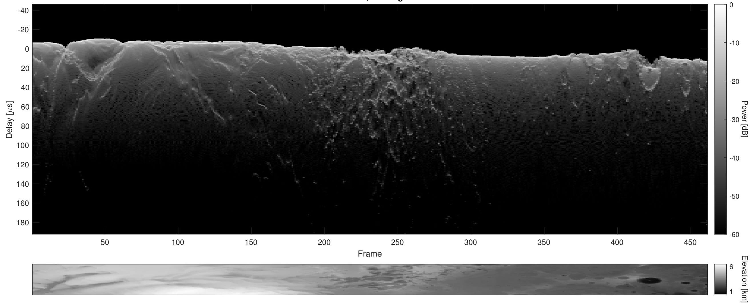
Orbit 23165, Cluttergram
