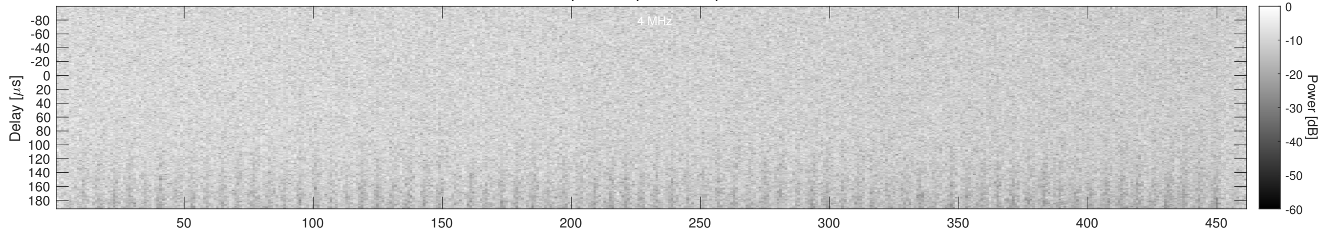
Orbit 23165, Window, Channel 2, Chapman
