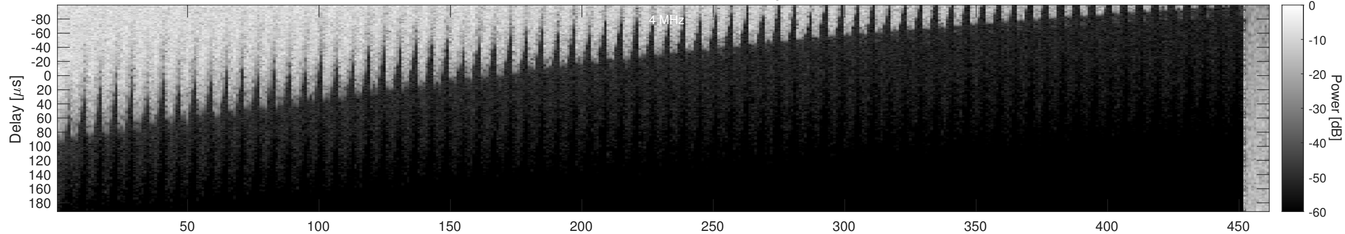
Orbit 23165, Window, Channel 2, Optimized
