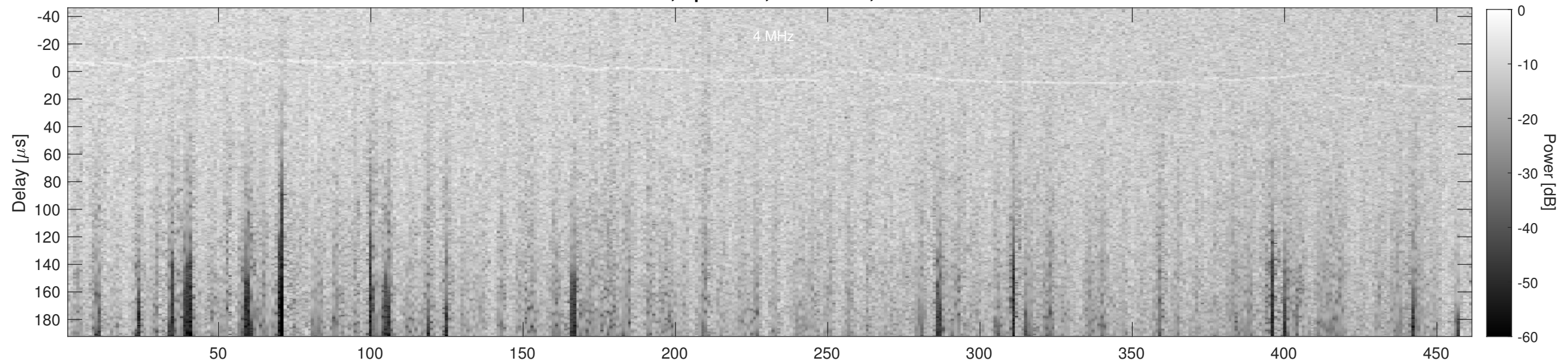
Orbit 23165, Cluttergram
