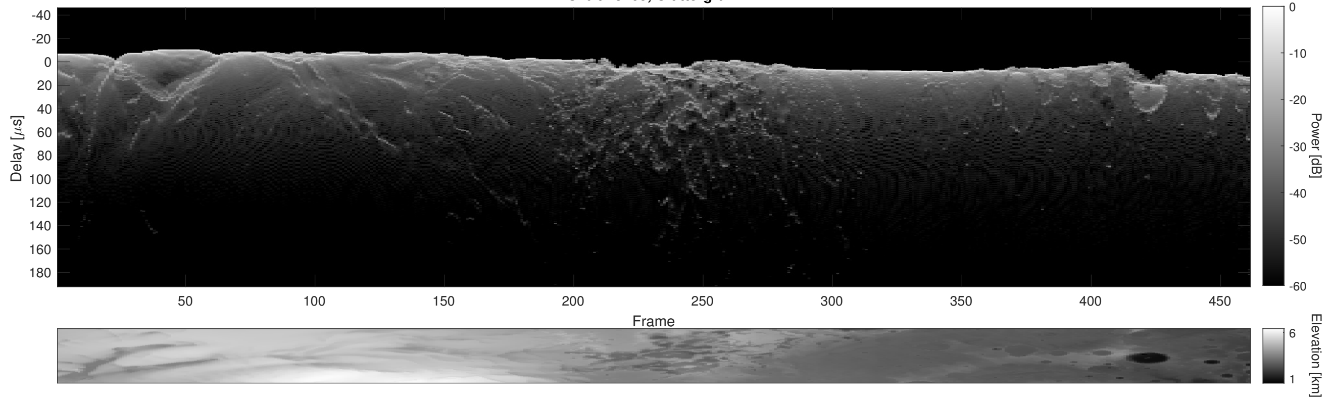
Orbit 23165, Cluttergram
