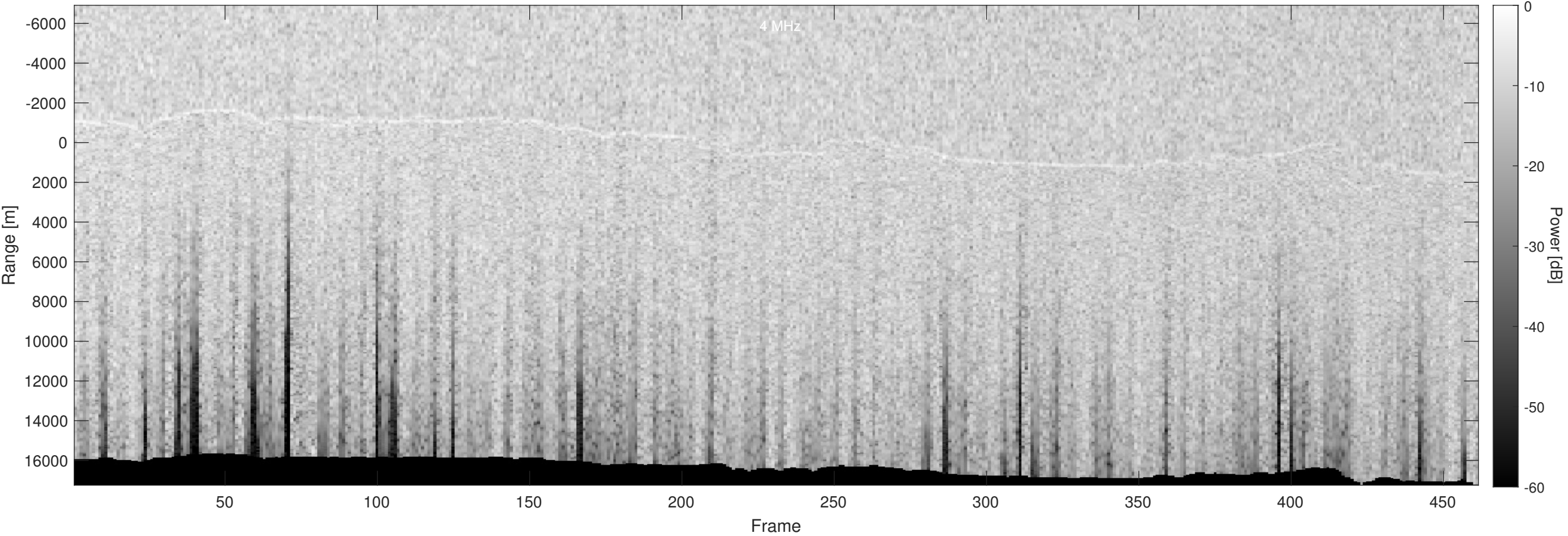
Orbit 23165, Optimized, Window, Depth-Corrected, Channel 2
