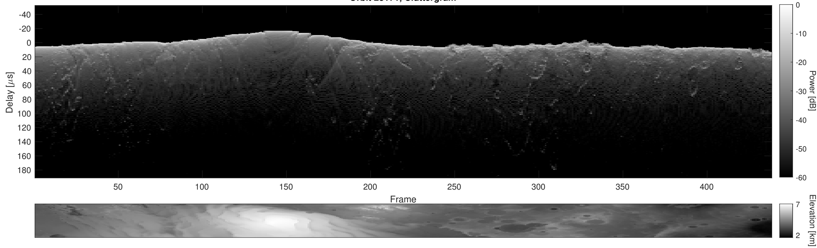
Orbit 23171, Cluttergram
