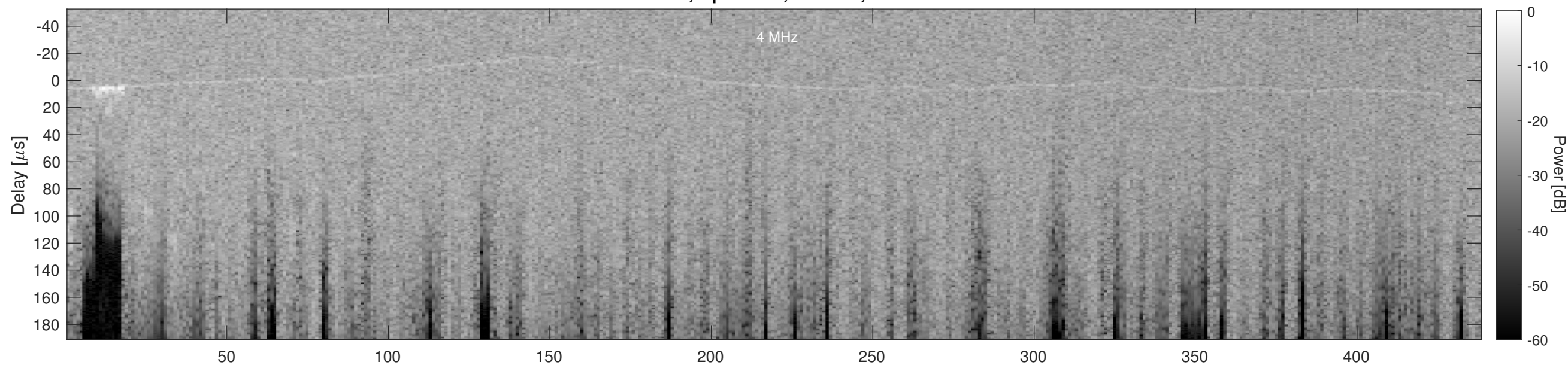
Orbit 23171, Cluttergram
